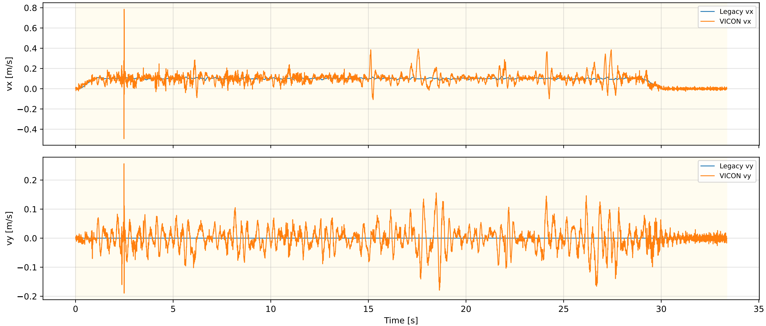
Legacy Odometry Velocity — RUGG_WLW_OLD_REAL_1
