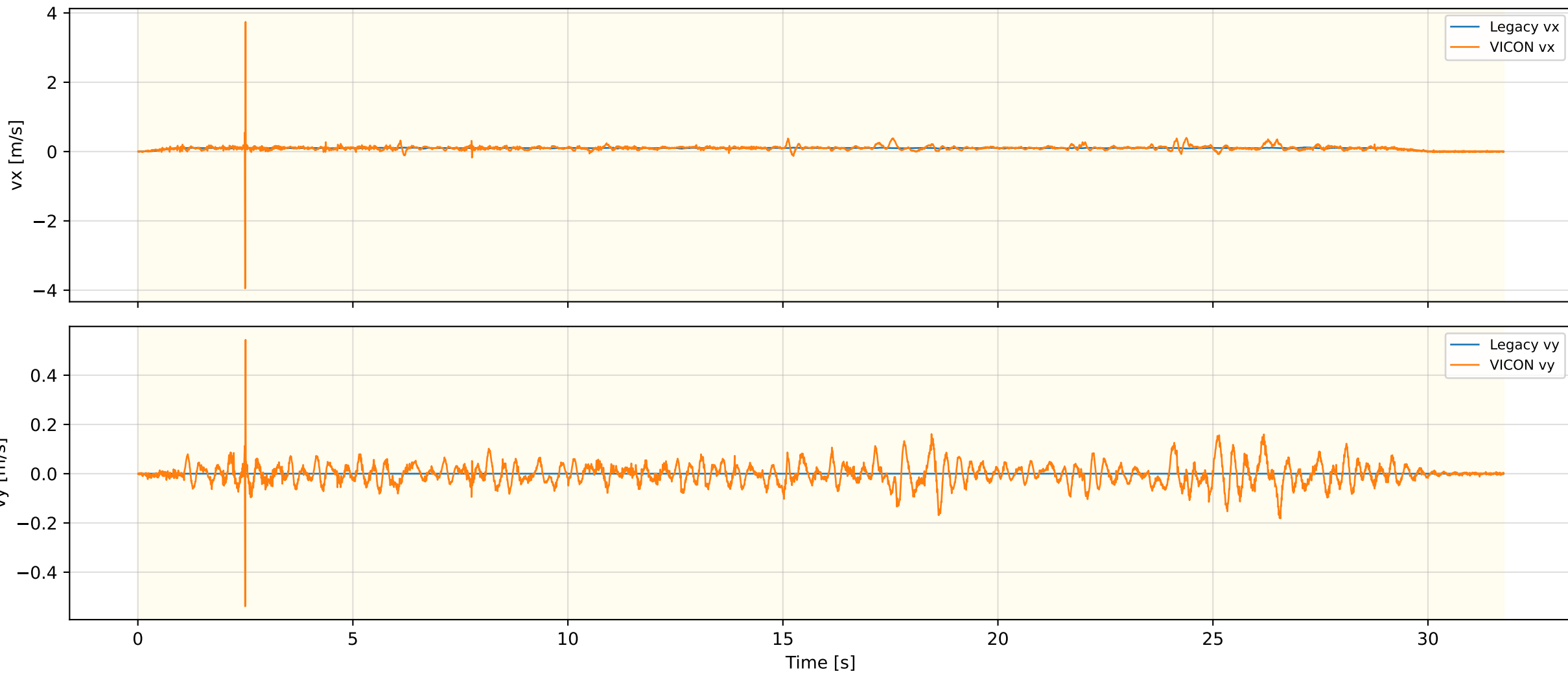
Legacy Odometry Velocity — RUGG_WLW_OLD_REAL_2
