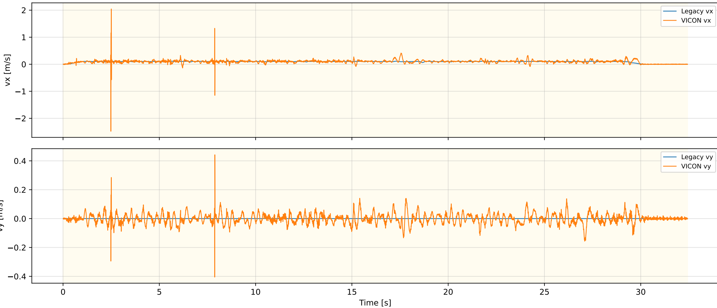
Legacy Odometry Velocity — RUGG_WLW_OLD_REAL_3
