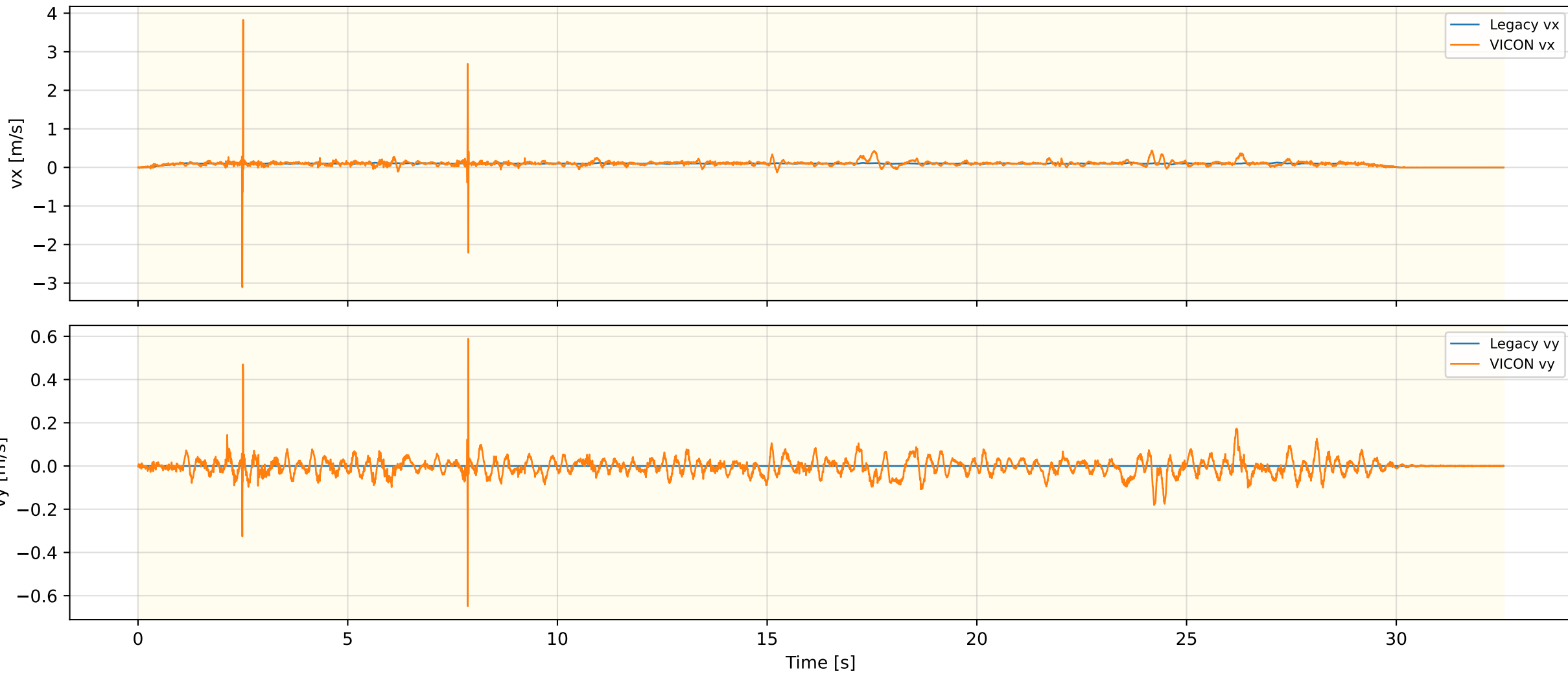
Legacy Odometry Velocity — RUGG_WLW_OLD_REAL_4
