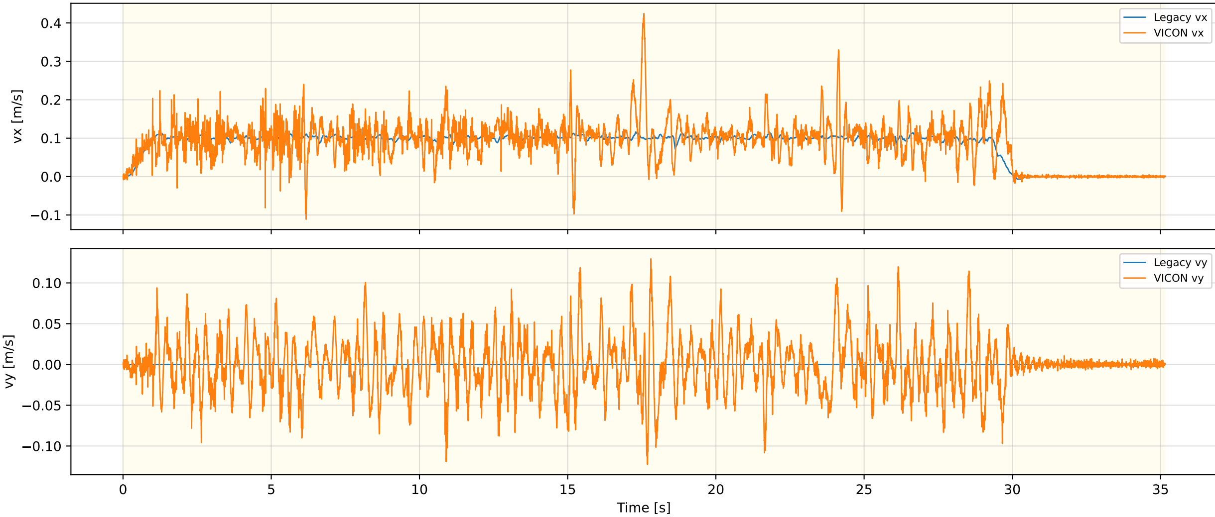
Legacy Odometry Velocity — RUGG_WLW_OLD_REAL_5
