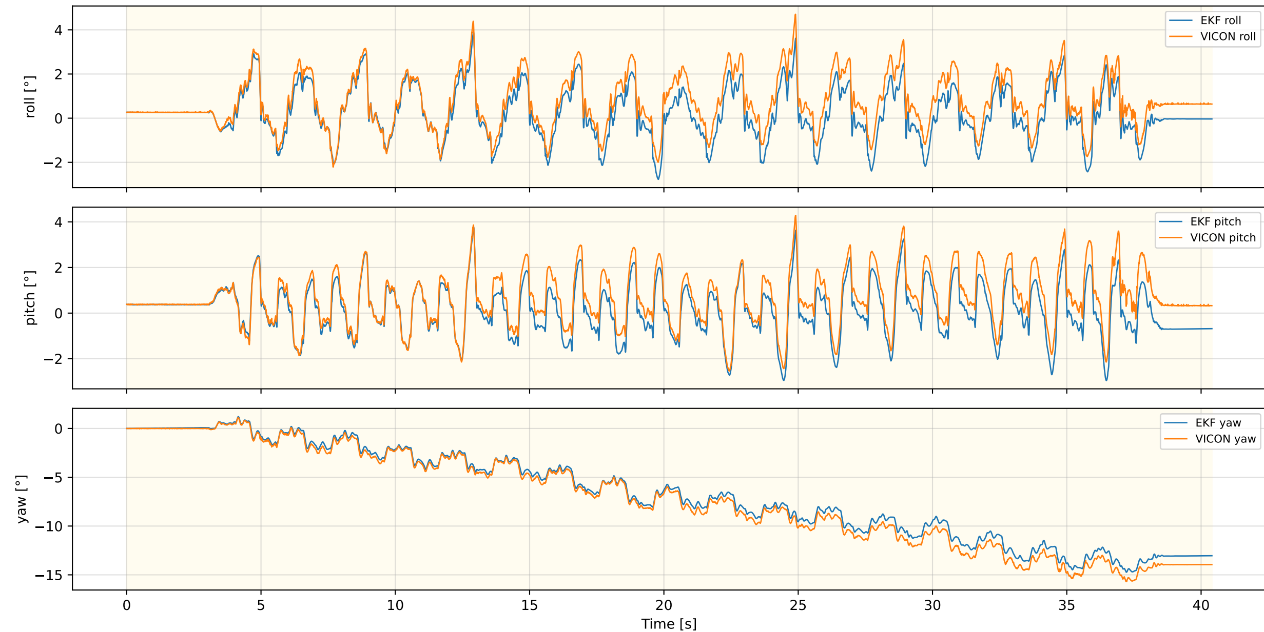
Inner EKF Attitude — FLAT_MPC_NEW_REAL_1
