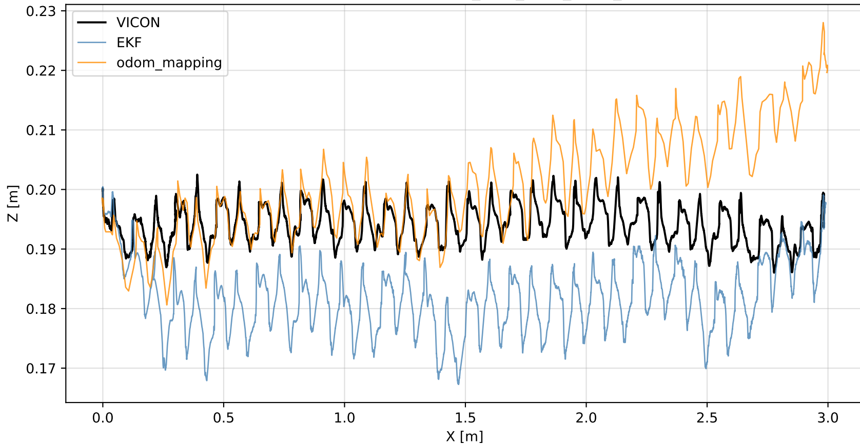
XZ Trajectory — FLAT_MPC_NEW_REAL_2
