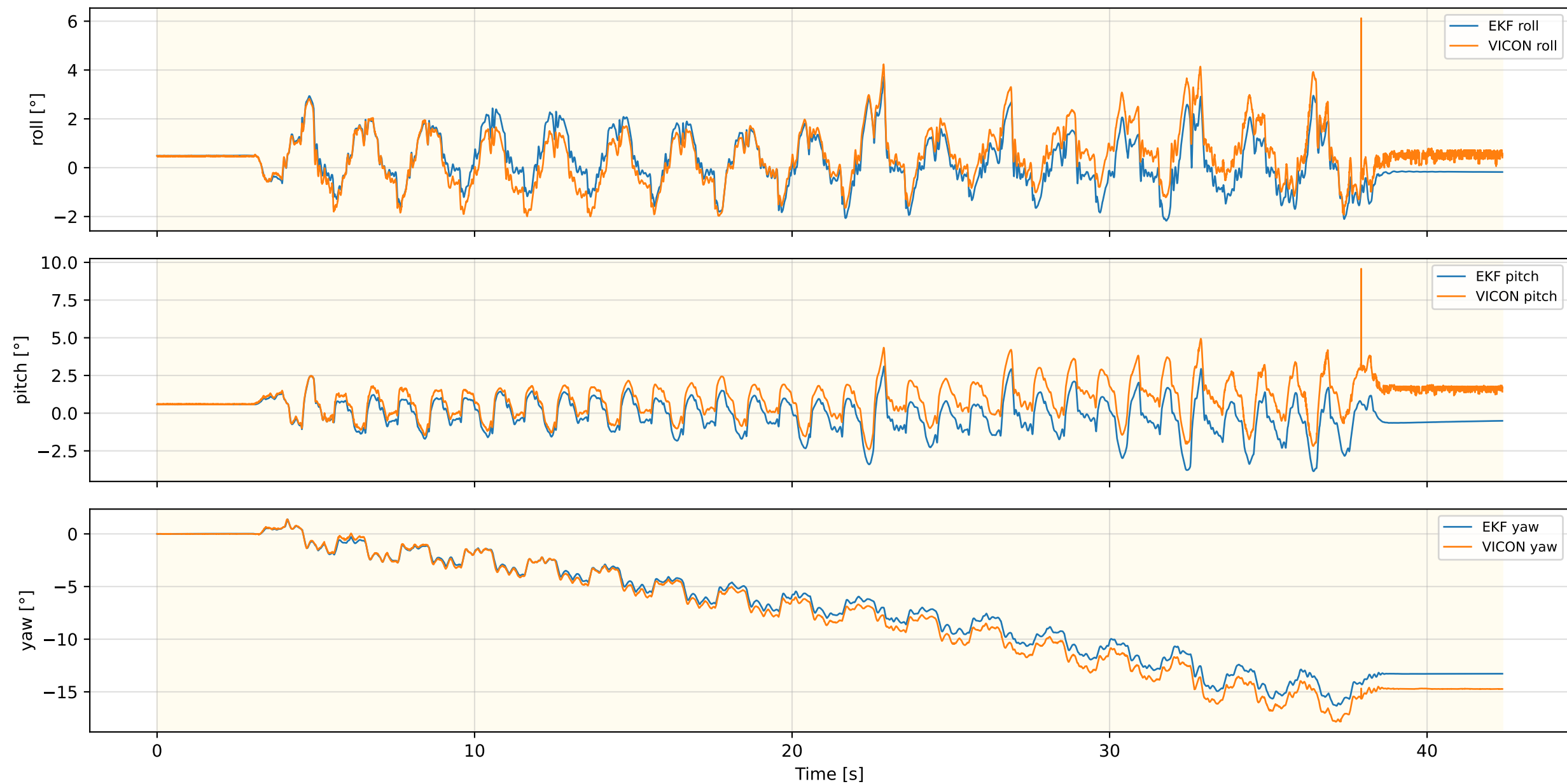
Inner EKF Attitude — FLAT_MPC_NEW_REAL_4
