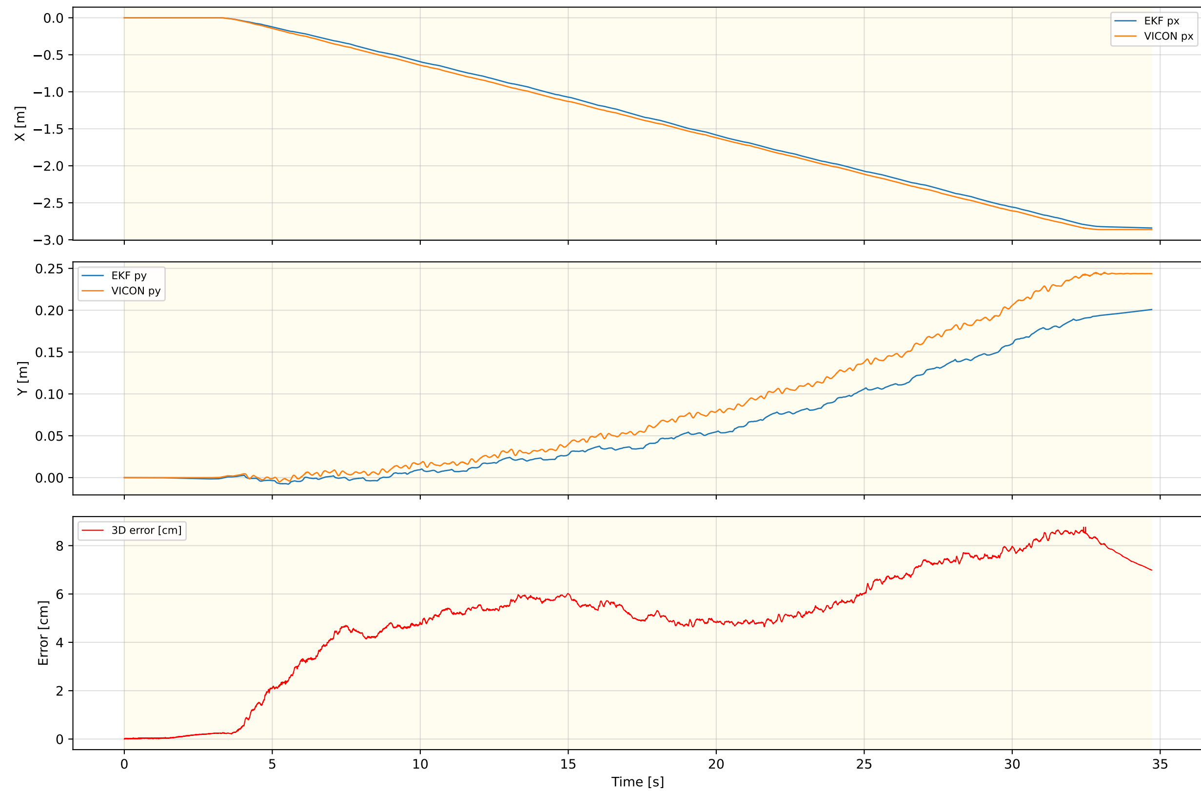
Inner EKF Position — FLAT_WLW_NEW_REAL_4
