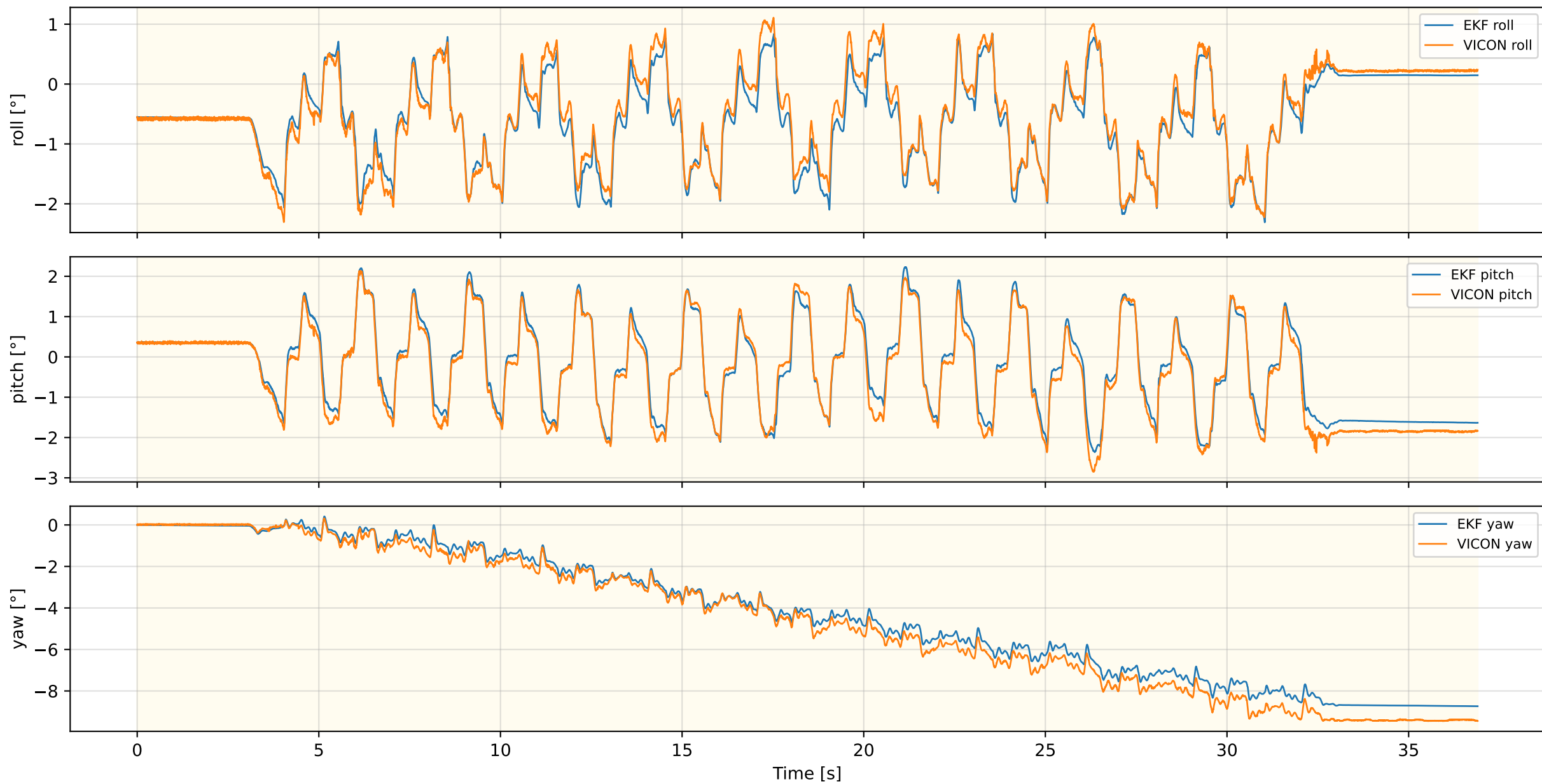
Inner EKF Attitude — FLAT_WLW_NEW_REAL_5
