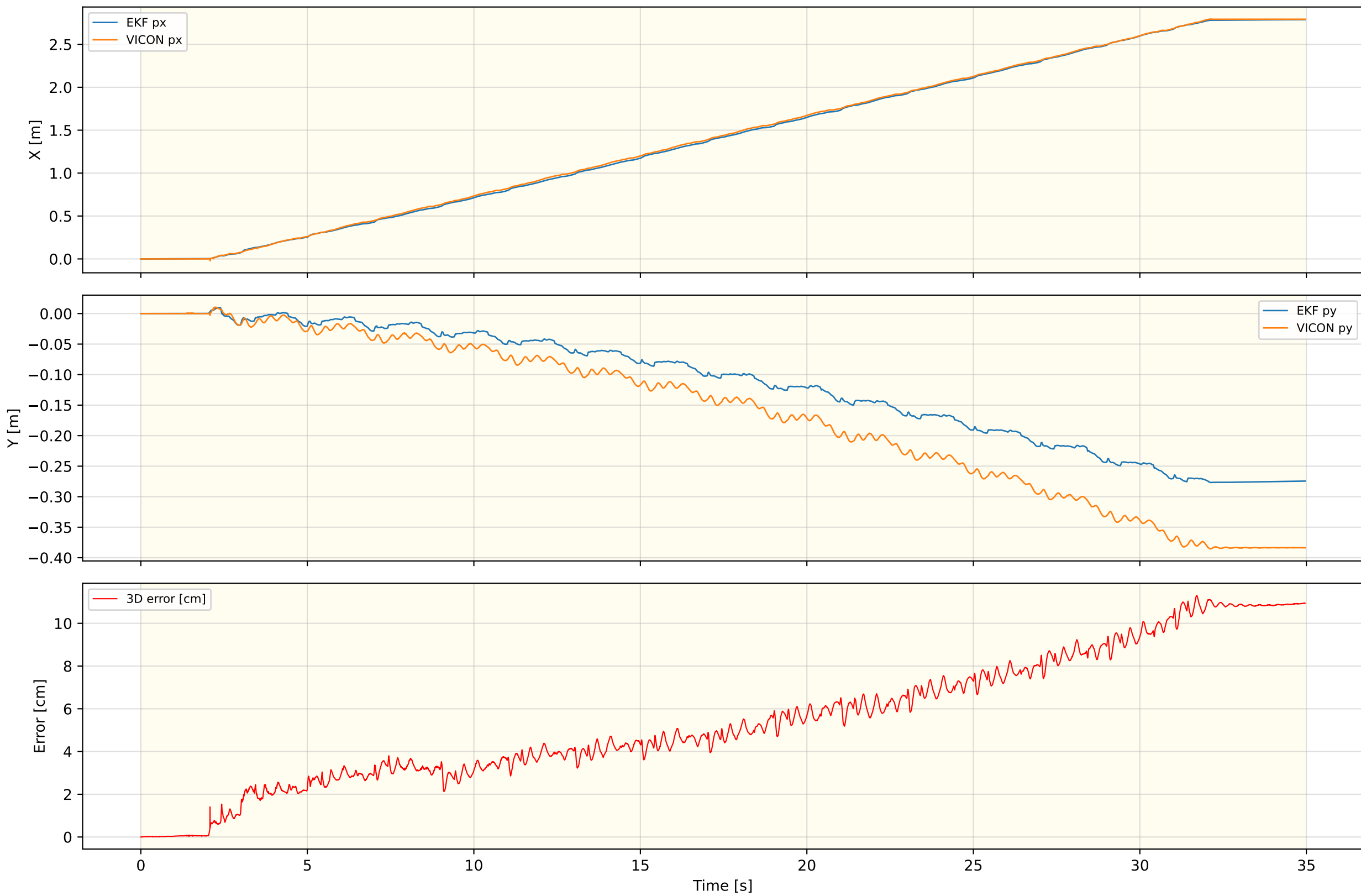
Inner EKF Position — FLAT_Walk_NEW_REAL_4
