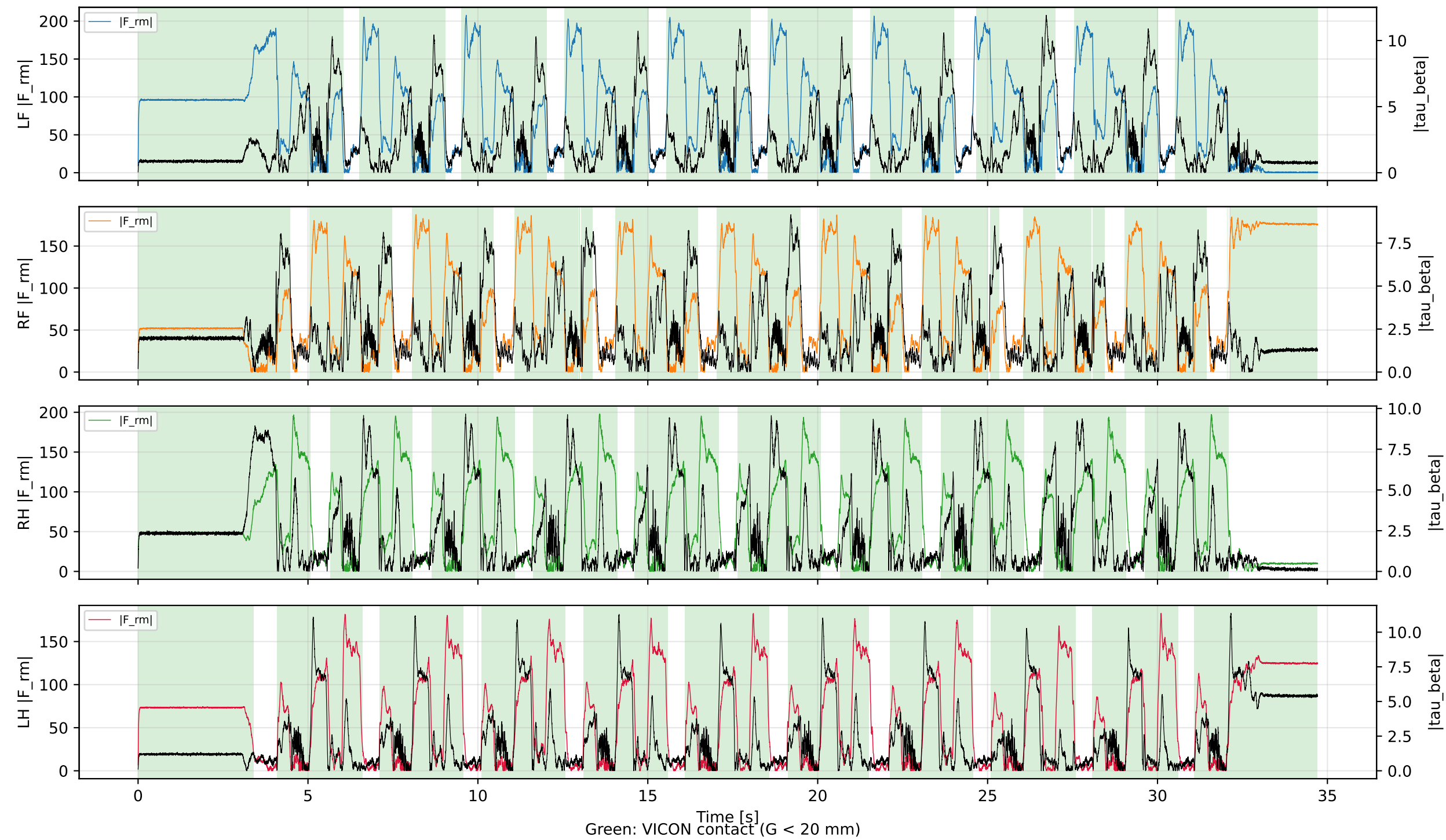
GMO Residuals vs VICON Ground Truth — FLAT_WLW_NEW_REAL_4
