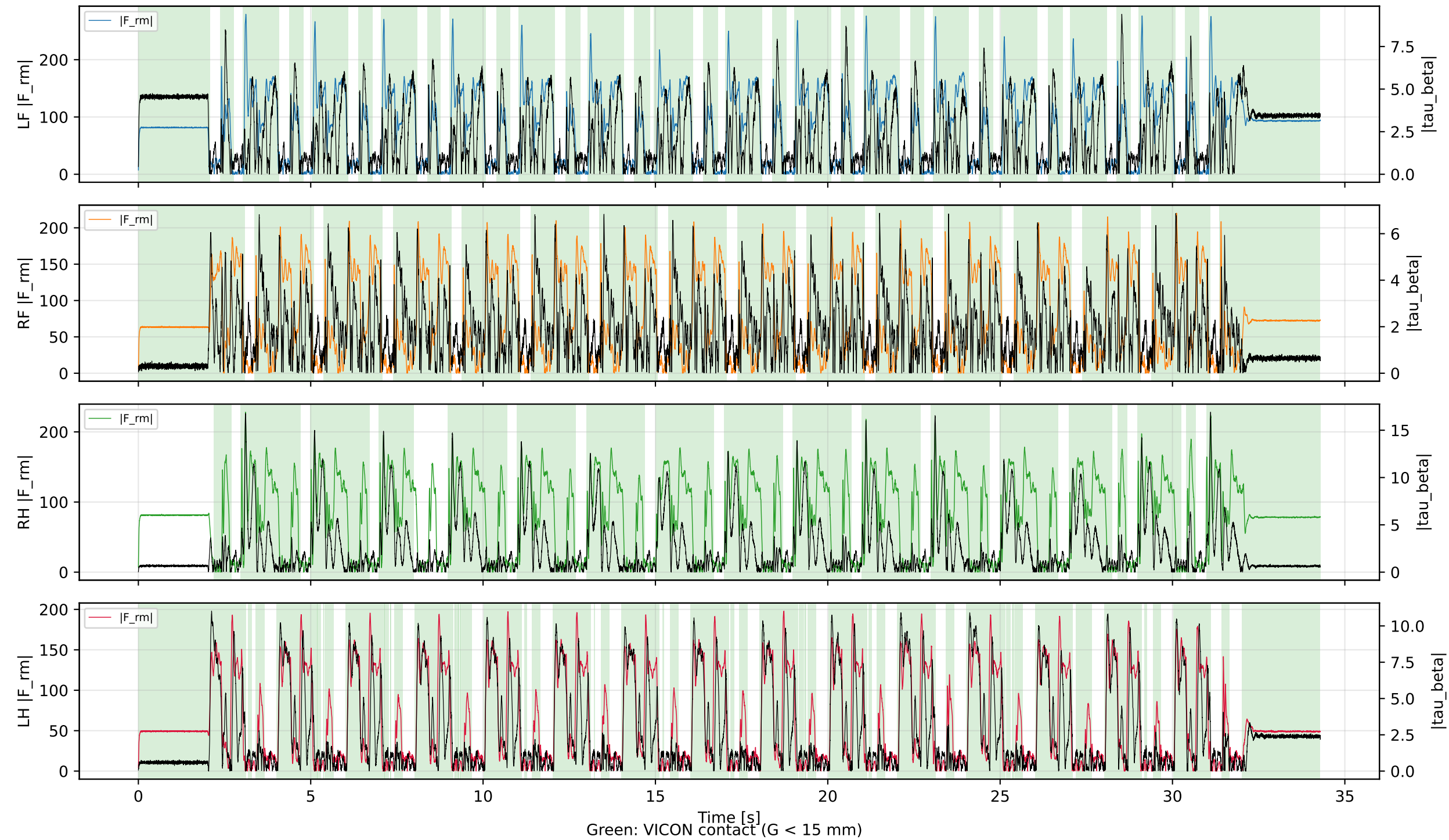
GMO Residuals vs VICON Ground Truth — FLAT_Walk_NEW_REAL_5
