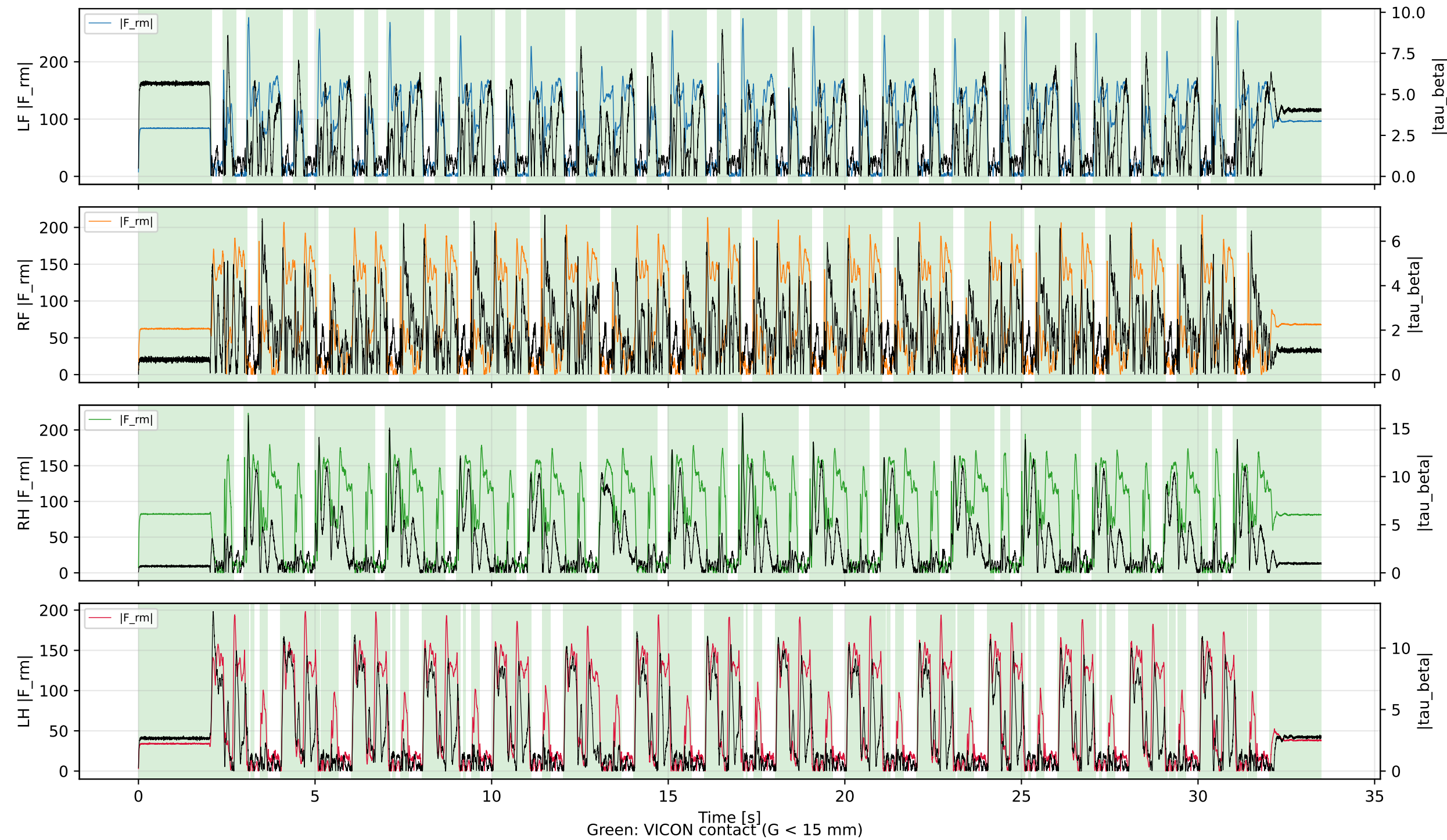
GMO Residuals vs VICON Ground Truth — FLAT_Walk_NEW_REAL_6
