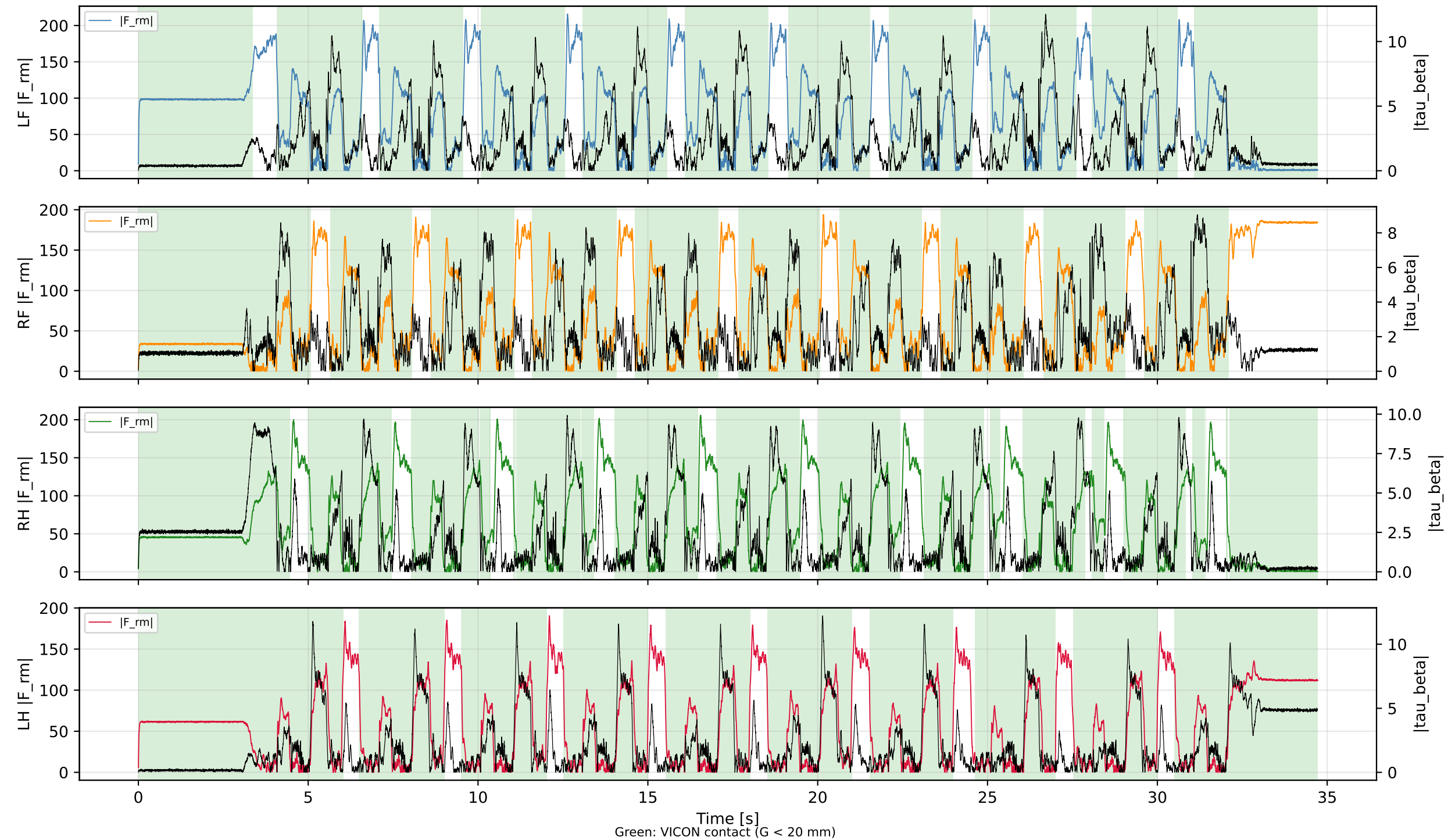
GMO Residuals vs VICON Ground Truth — FLAT_WLW_NEW_REAL_1
