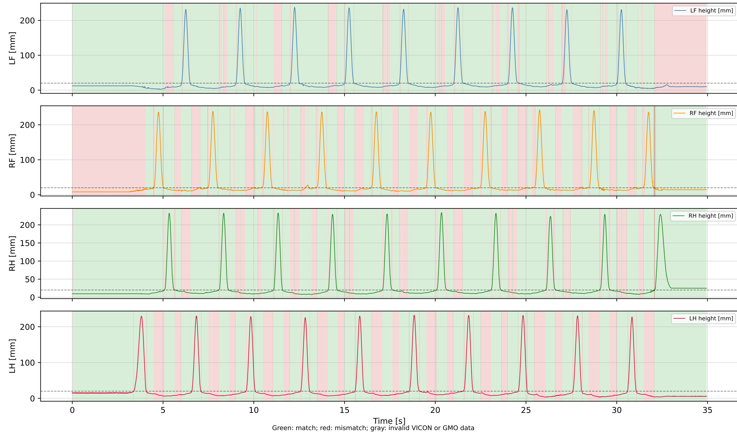
Contact Detection — FLAT_WLW_NEW_REAL_2 (VICON < 20 mm; F_rm 50/25, tau_beta 3.00/1.50)
