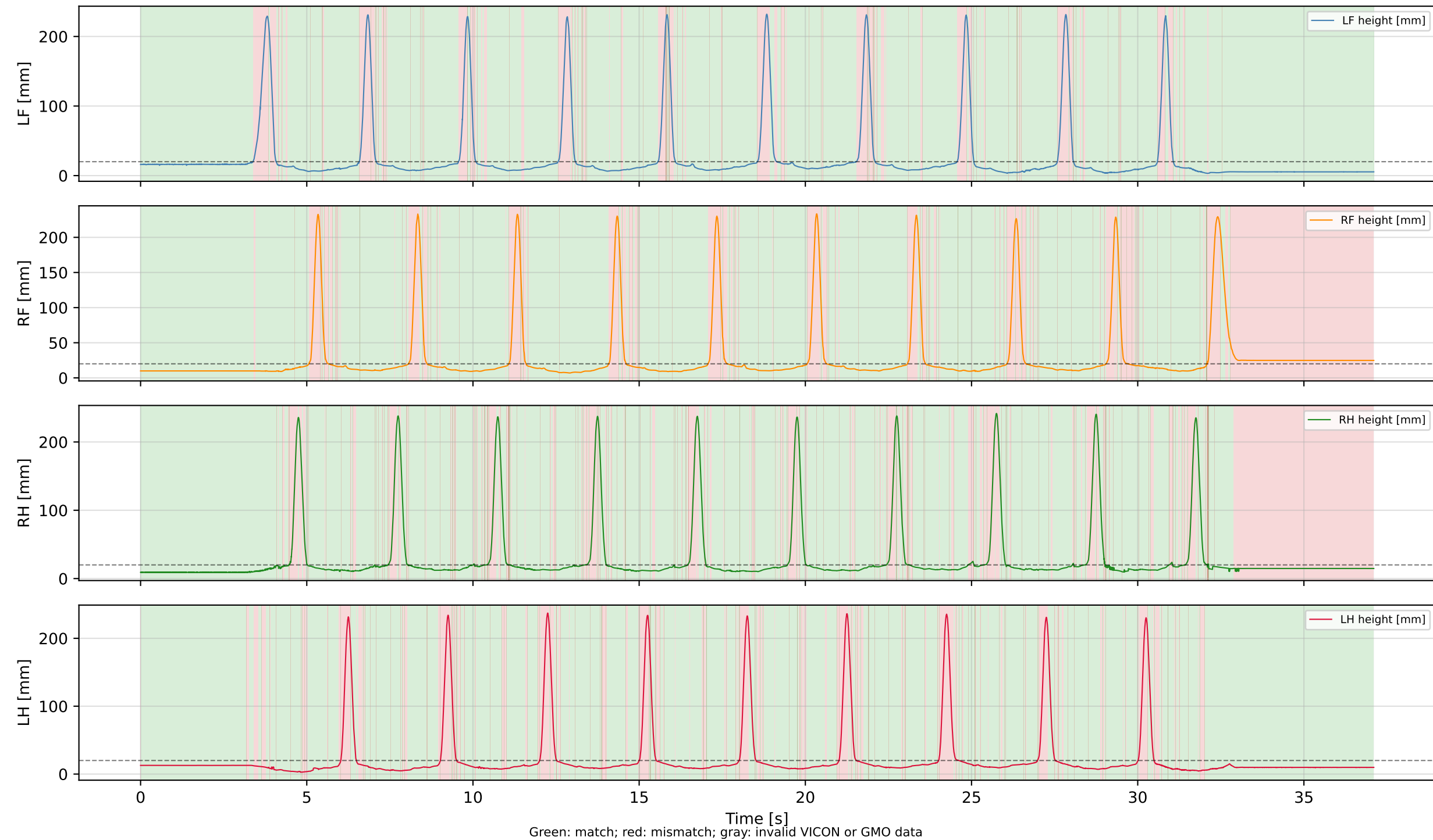
Contact Detection — FLAT_WLW_NEW_REAL_3 (VICON < 20 mm; F_rm 225/205, tau_beta 0.50/0.25)
