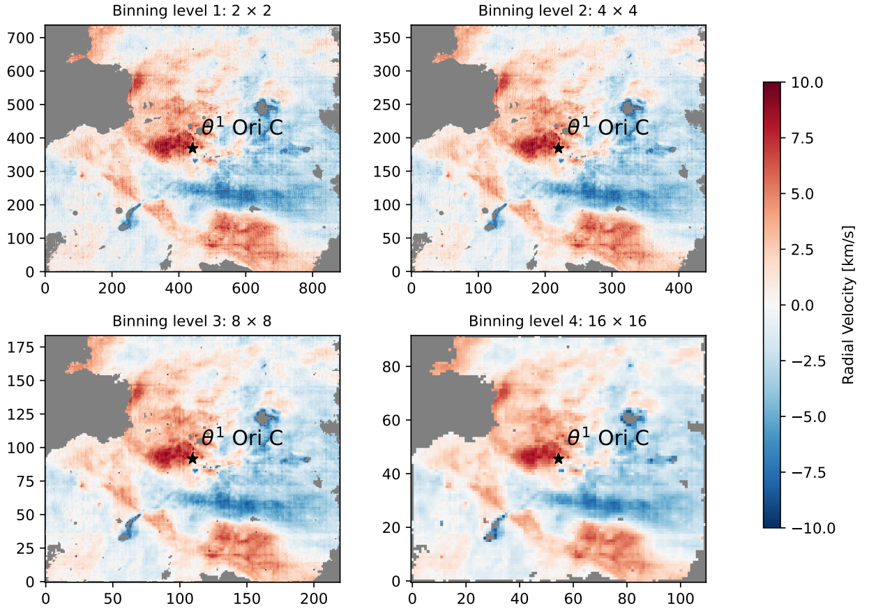
Figure 4. Two-dimensional binned maps of the centroid velocity of the Orion nebula for the H\alpha emission line. The size of each map are 737 \times 882 , 368 \times 440 , 183 \times 219 and 91 \times 109 pixels which correspond to the bin sizes of 2^1 = 2 , 2^2 = 4 , 2^3 = 8 and 2^4 = 16 respectively. The same procedure of binning is applied to all emission lines.
