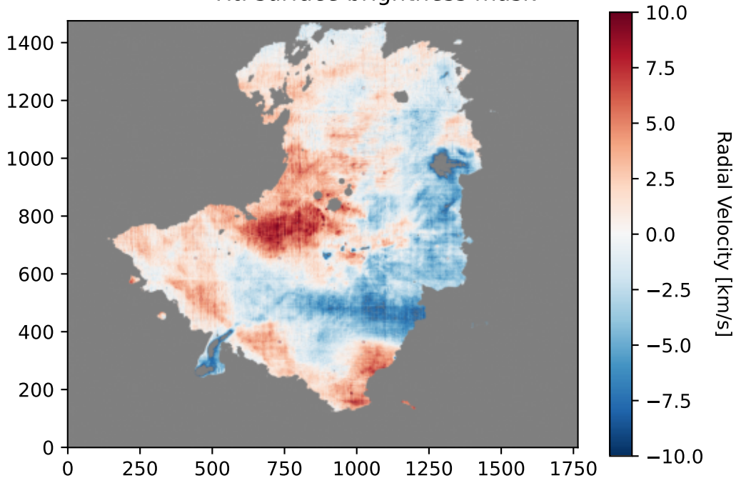
H \alpha surface brightness mask
