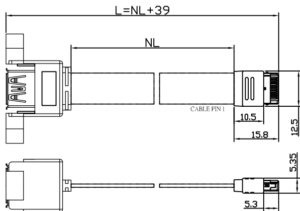
CABLE: UL21099/UL21283/UL21425 /UL22112/EQUIVALENT 21P 30AWG, BLACK
