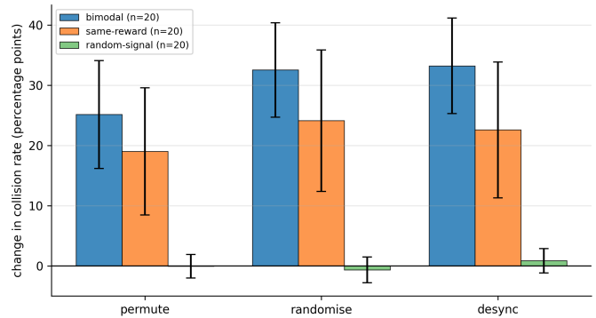
Fig. 8: Change in collision rate under the three token-corrupting interventions, by training family. Bars are means over the 20 seeds of each family and error bars are 95% seed-level confidence intervals on the paired difference from that family’s own baseline. The penalty tracks whether a family had learned to use the token: large in the bimodal, smaller in the same-reward, and absent in the random-signal, whose agents never bound the token to behaviour.
