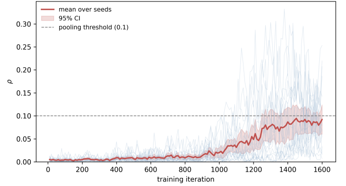
Fig. 4: \rho over training for the bimodal condition. Faint lines are the 20 individual seeds; the solid line is the mean, and the shaded band is the 95% seed-level confidence interval at each logged iteration; the dashed line marks the pooling threshold \rho = 0.1 .
