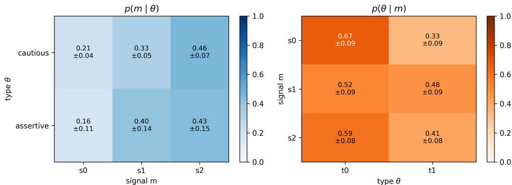
Fig. 6: Signal use in the bimodal condition, mean over 20 seeds. Left: p(m | \theta) , how each type distributes its tokens. Right: p(\theta | m) , the type implied by a received token. Error terms are 95% seed-level confidence intervals per cell.
