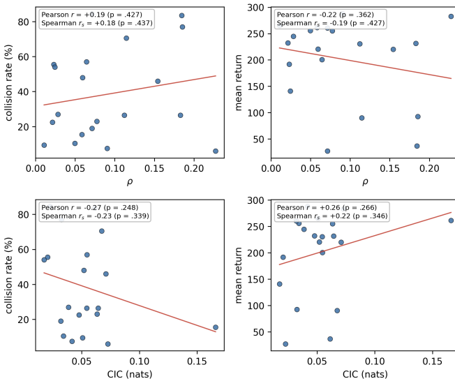
Fig. 11: Seed-level relationships between the signalling metrics ( \rho , CIC) and task outcomes (collision rate, mean return) across 20 bimodal seeds. Each point is one seed and the line is an ordinary least-squares fit. Each panel is annotated with the Pearson r and the Spearman r_s over the 20 seeds, with the associated p -value. All four relationships are weak and none is significant.
