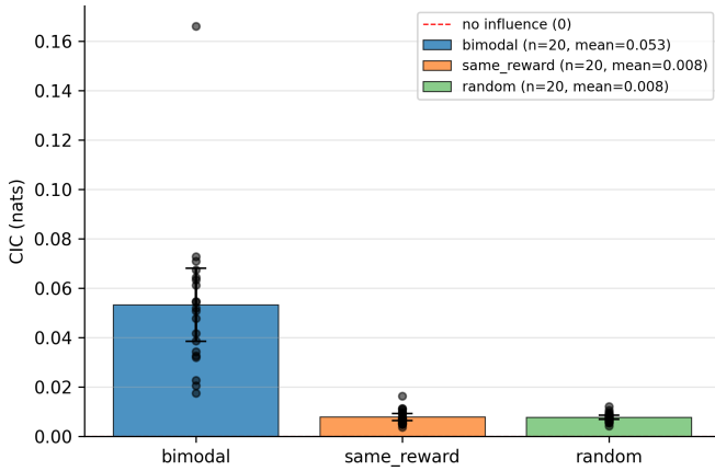
Fig. 10: Causal Influence of Communication by condition (nats). Bars are means over the 20 seeds, error bars are 95% seed-level confidence intervals, and points are individual seeds.
