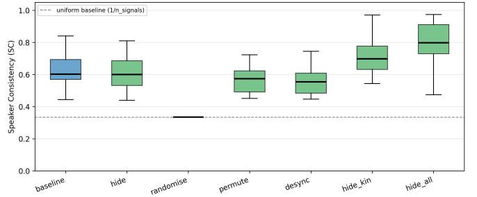
Fig. 5: Speaker Consistency by intervention, bimodal family. The dashed line marks the chance level 1/|\mathcal{M}| = 0.33 .
