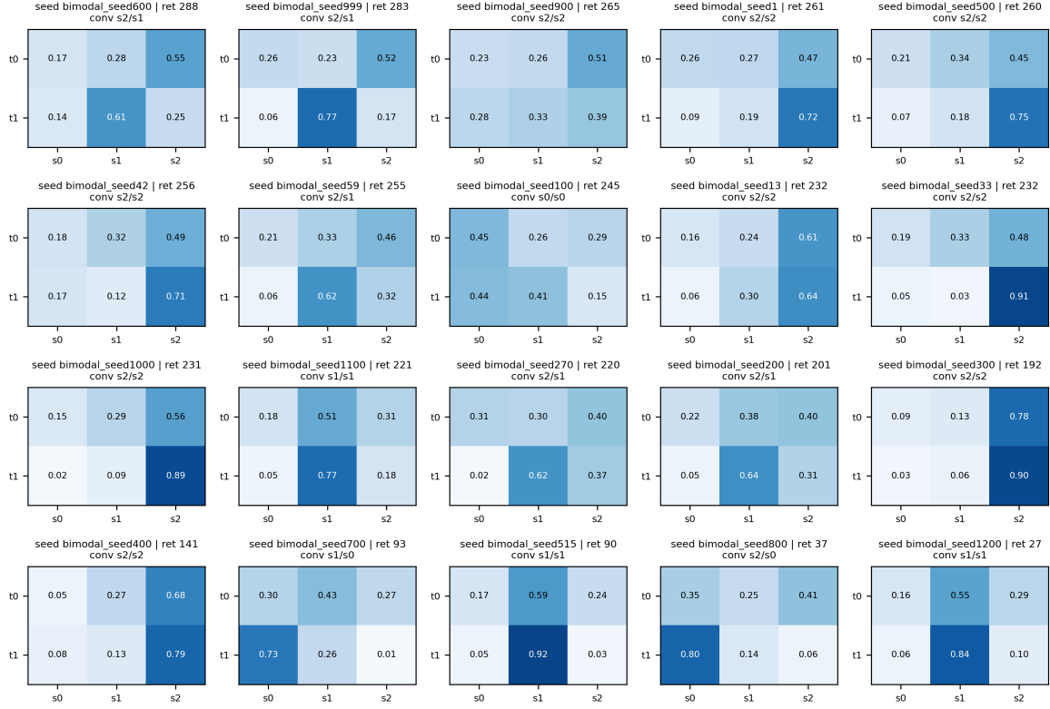
Fig. 12: Signal heatmap by seed in the bimodal condition, sorted by descending mean return.
