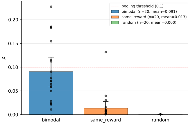
Fig. 3: Separation coefficient \rho by condition. Bars are means over 20 seeds with 95% seed-level confidence intervals; points are individual seeds.
