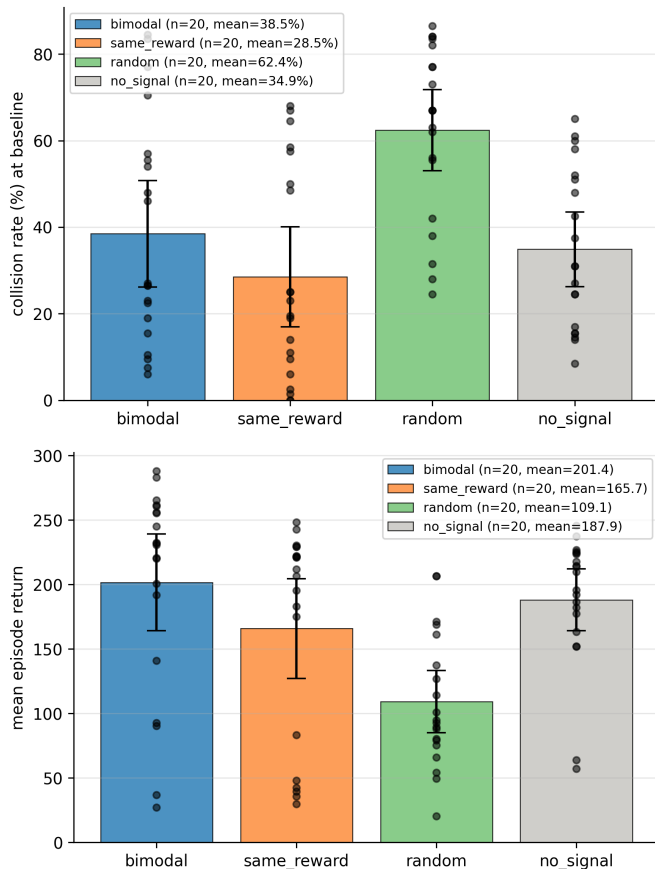
Fig. 7: Collision rate and return by condition under the unmodified baseline. Top: the collision rate. Bottom: the mean episode return. Bars are means over the 20 seeds of each condition, error bars are 95% seed-level confidence intervals, and points are individual seeds.
