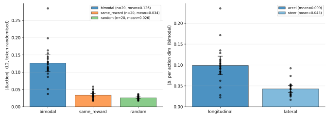
Fig. 9: Counterfactual Decoding Effect across conditions. Left: change in the receiver’s mean action when the received token is altered with the scene frozen, by condition. Right: per-dimension change in the bimodal family. Bars are means over the 20 seeds, error bars are 95% seed-level confidence intervals, and points are individual seeds.
