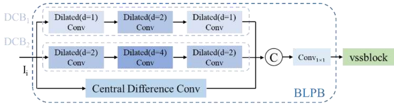
Fig. 2: Details of the LGSM module. It achieves multi-level feature extraction from local details to global semantics through the coordinated design of the Basic Local Perception Block (BLPB) and the Visual State Space Block (VSSBlock). The BLPB employs dilated convolutional branches (DCB) to dynamically enlarge the receptive field, while center difference convolution is integrated to enhance edge responses to weak and small targets.
