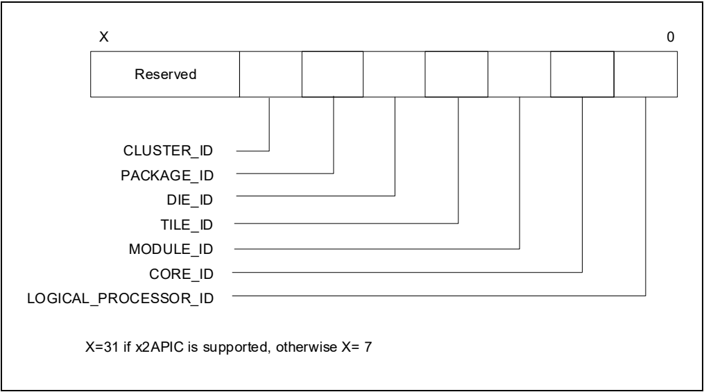
Figure 11-5. Generalized Seven-Domain Interpretation of the APIC ID
