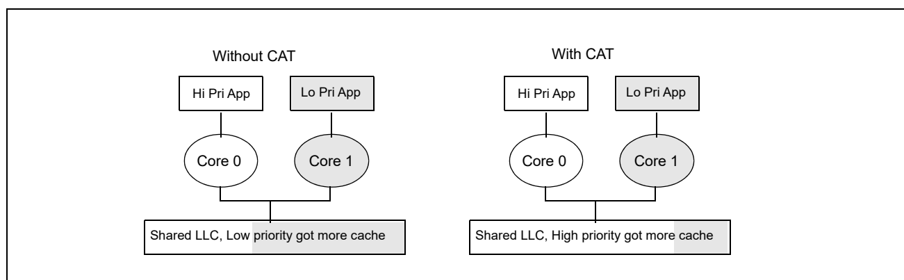
Figure 20-26. Cache Allocation Technology Enables Allocation of More Resources to High Priority Applications
