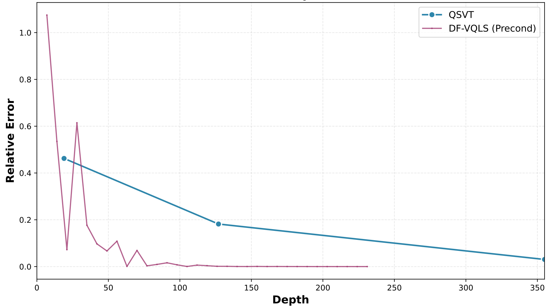
QSVT vs DF-VQLS Comparison (2×2, \kappa=3 )
