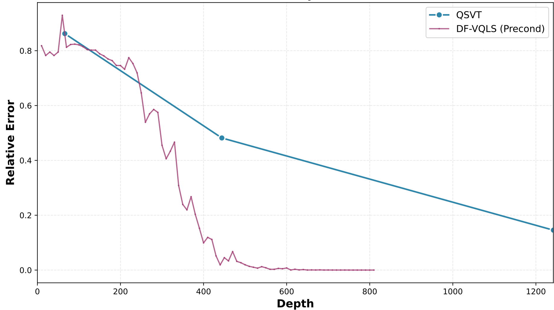
QSVT vs DF-VQLS Comparison (4×4, \kappa=3 )
