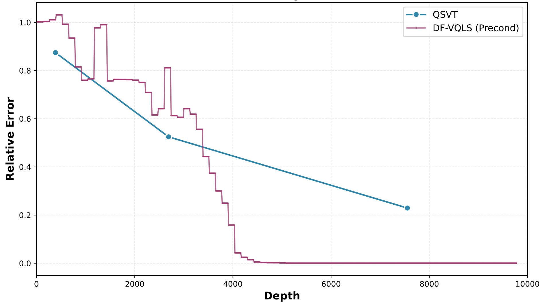
QSVT vs DF-VQLS Comparison ( 8 \times 8 , \kappa=4 )
