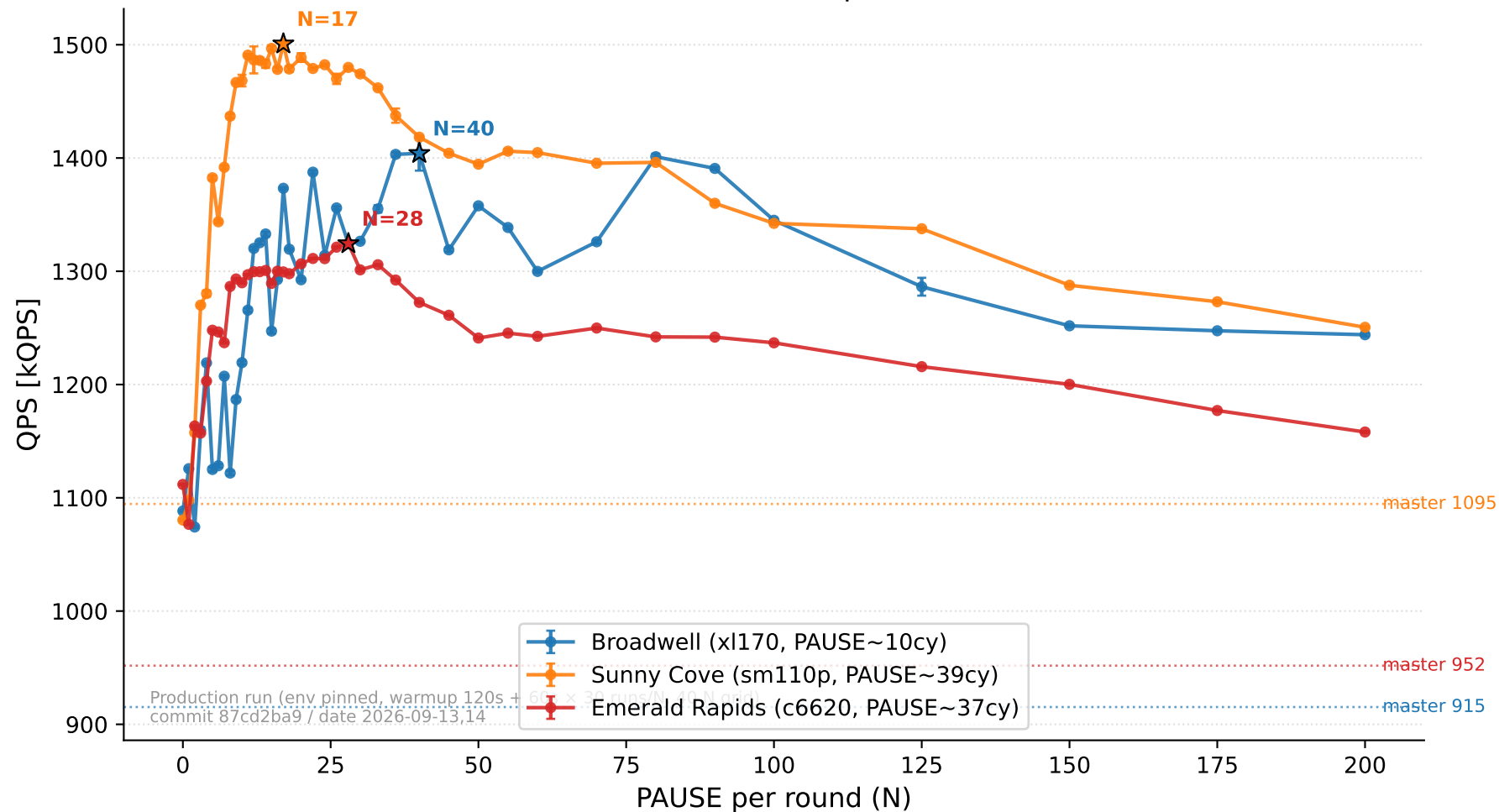
QPS vs N — 3 archs (production)
