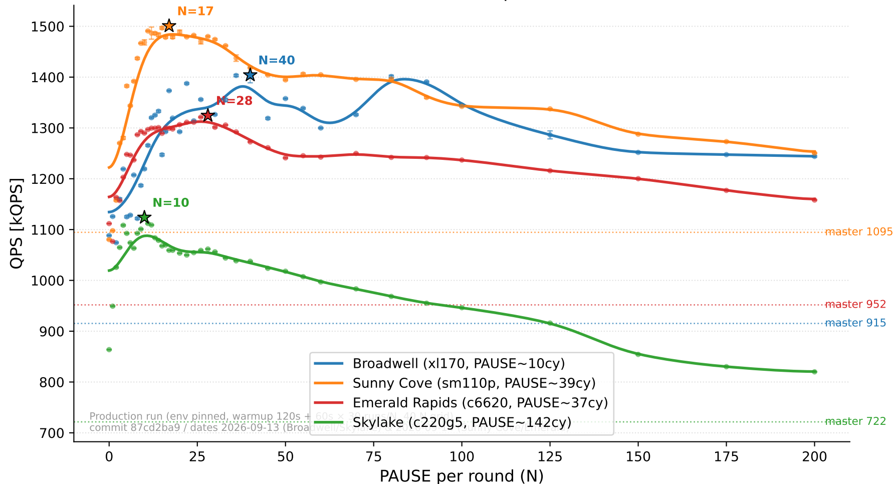
QPS vs N — 4 archs (production)
