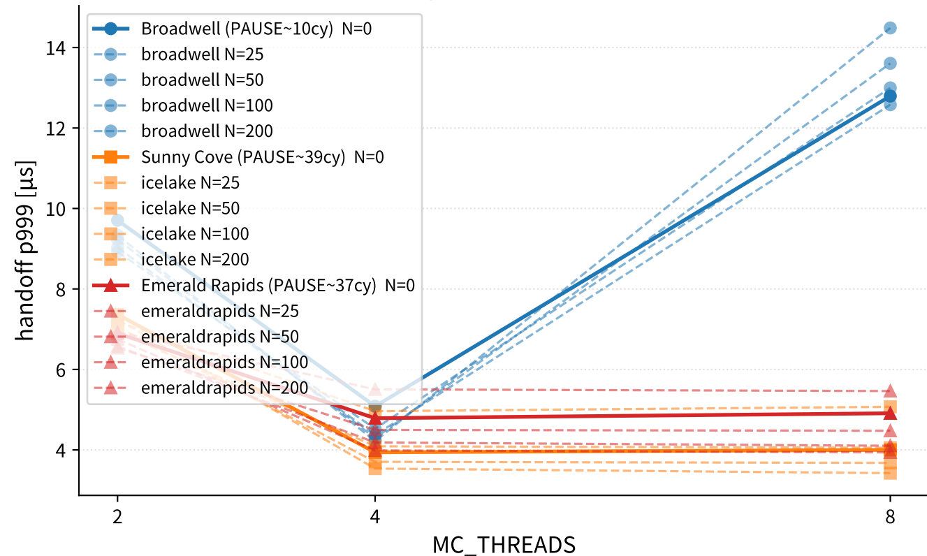
handoff p999 vs MC_THREADS
