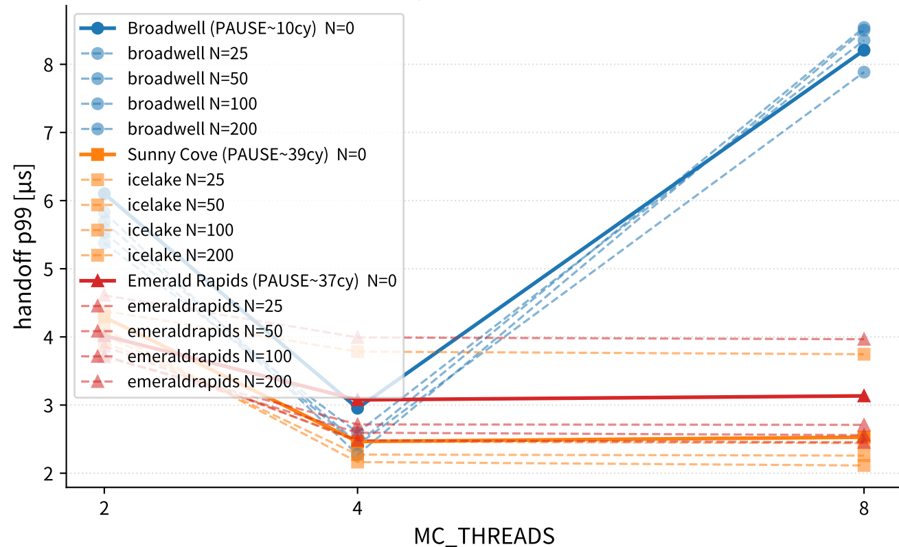
handoff p99 vs MC_THREADS
