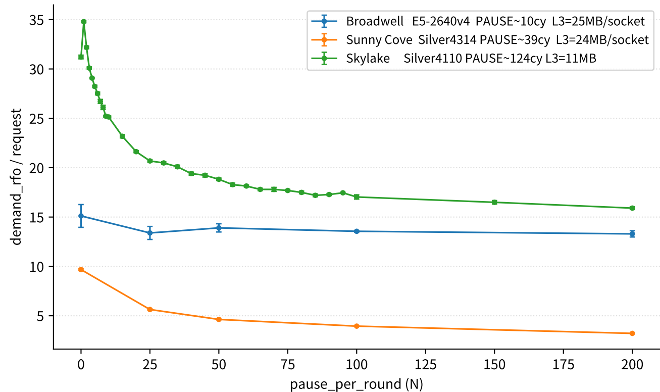
Bus contention (offcore RFO) vs PAUSE count
