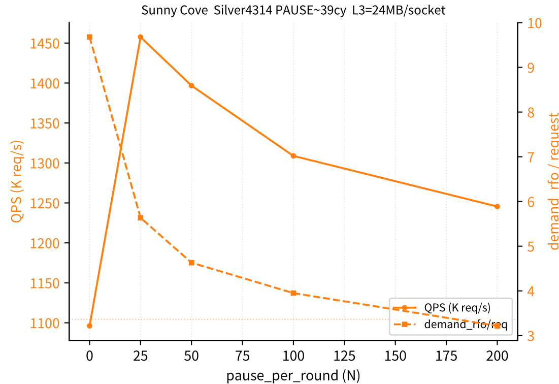
QPS and Bus Contention vs PAUSE count
