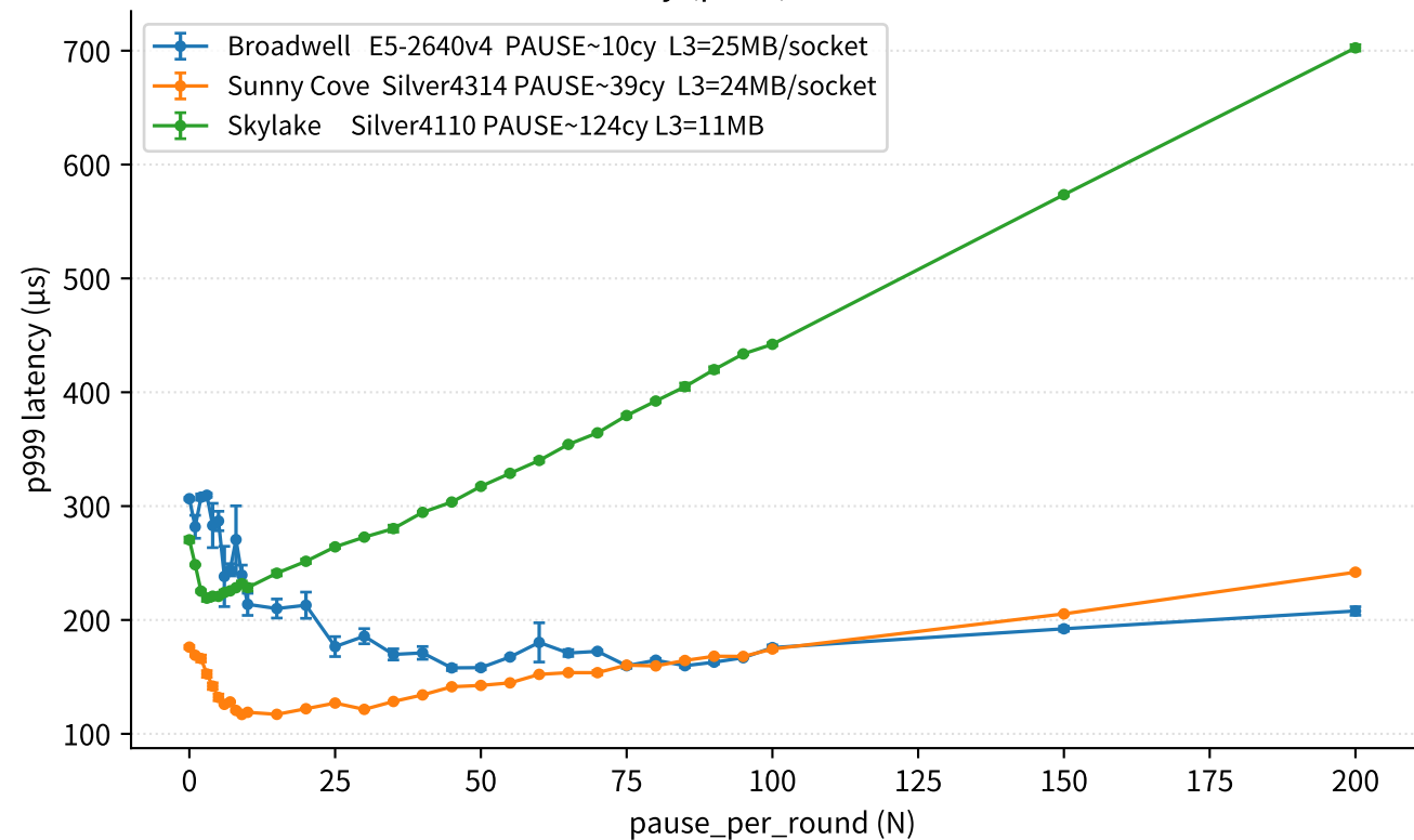
Tail latency (p999) vs PAUSE count
