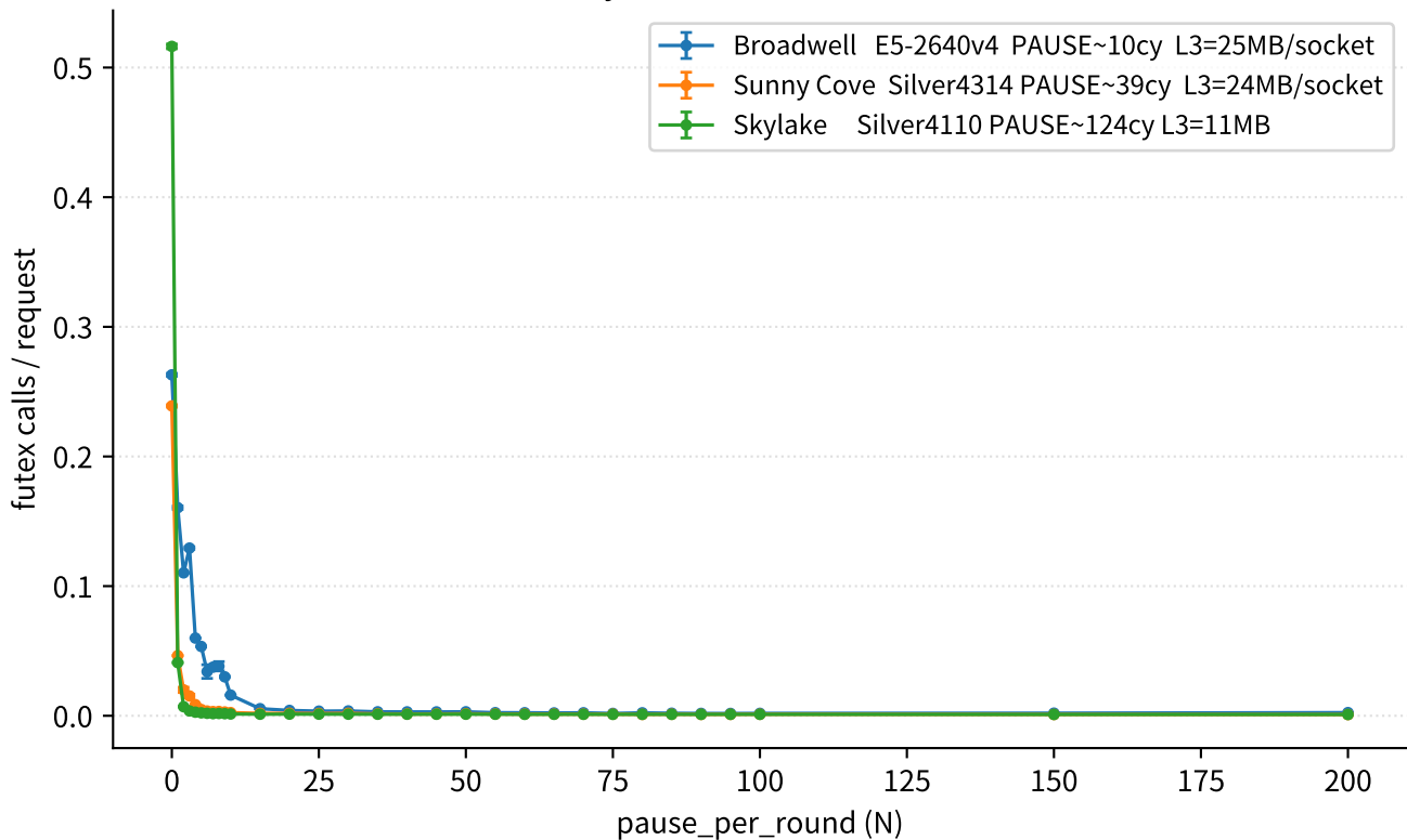
Futex syscall rate vs PAUSE count
