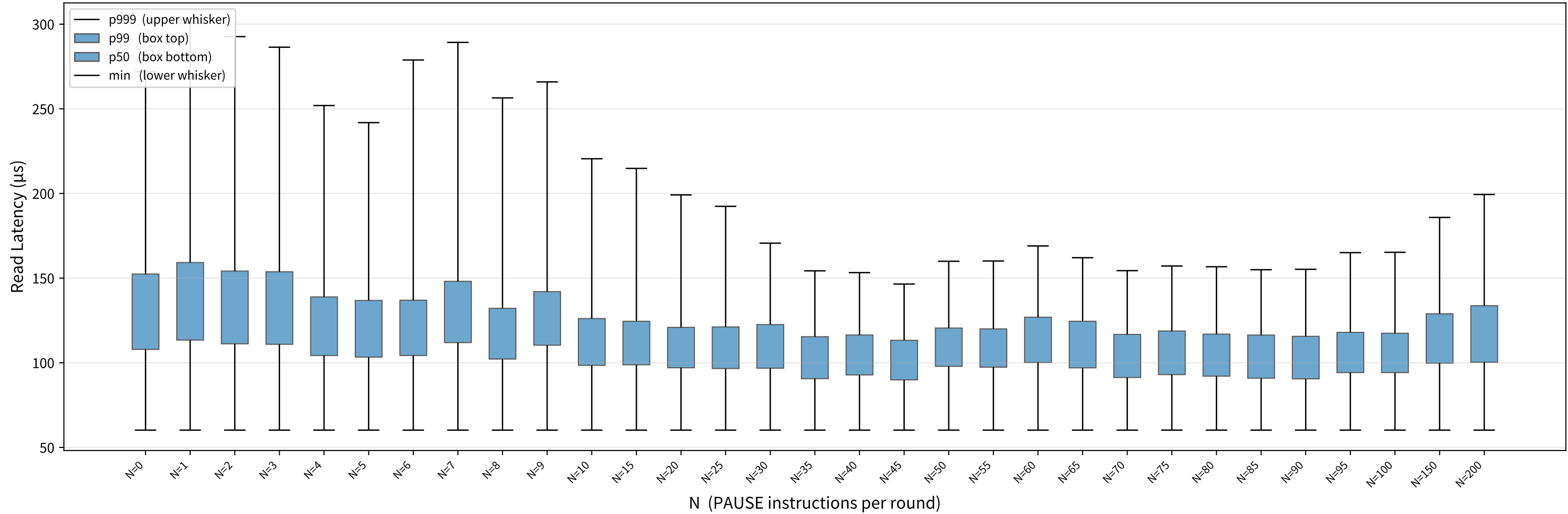
Broadwell (xl170, PAUSE~10cy) Read Latency [box: min / p50 / p99 / p999] / spinlock: [trylock→PAUSE×N]×30 / median across runs
