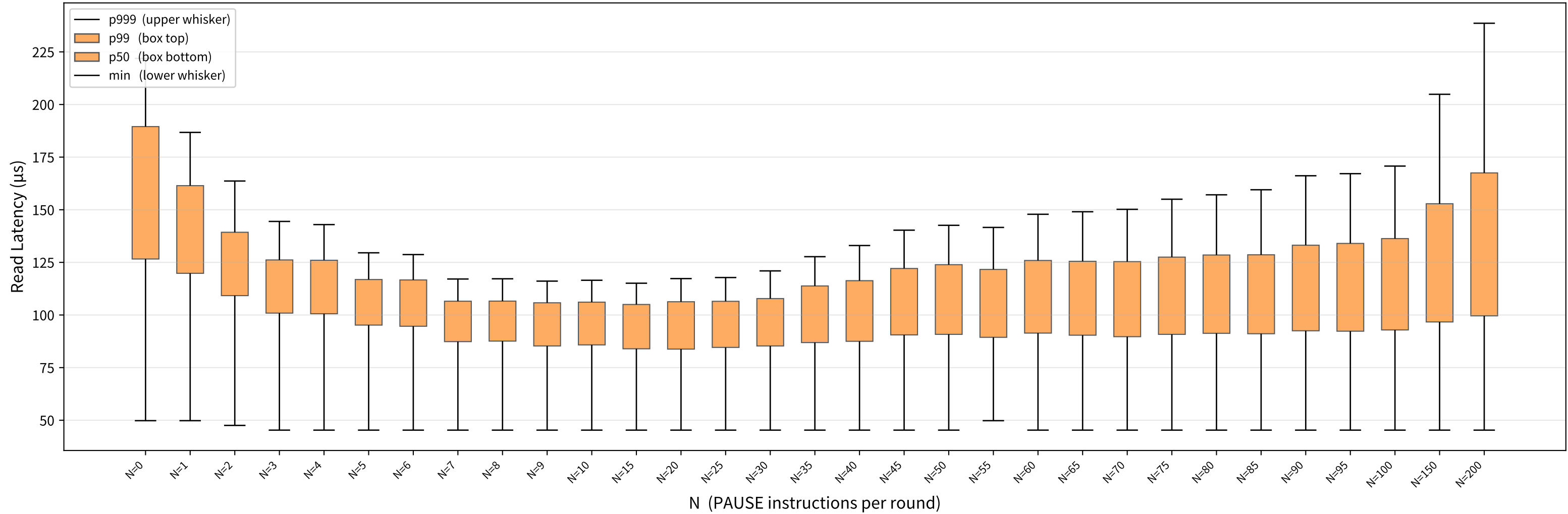
Ice Lake (sm110p, PAUSE~39cy) Read Latency [box: min / p50 / p99 / p999] / spinlock: [trylock→PAUSE×N]×30 / median across runs
