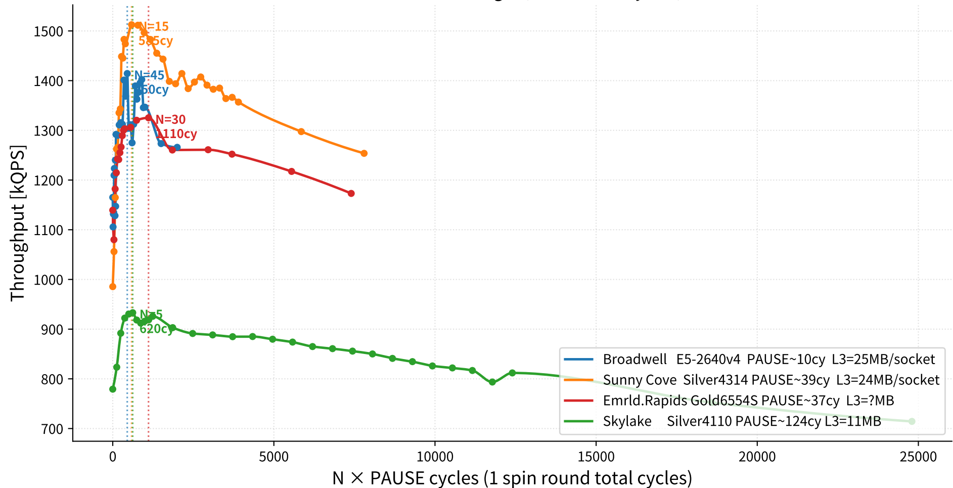
QPS vs PAUSE budget ( N \times \text{PAUSE cycles} )
