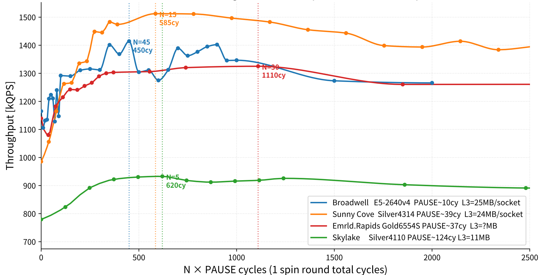
QPS vs PAUSE budget ( N \times PAUSE cycles) [zoom: 0-2500 cy]
