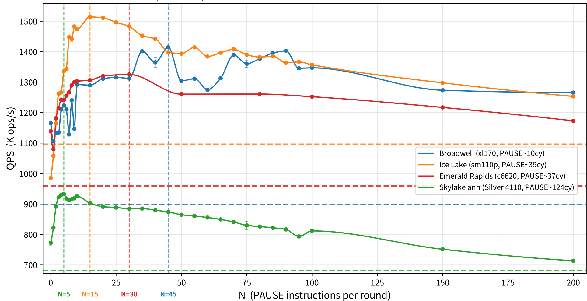
Throughput vs PAUSE count [cubic spline, error bar = CV%] spinlock: [trylock \rightarrow PAUSE \times N] \times 30 \rightarrow mutex_lock / mc=4t mut-T4 -c1 -d32
