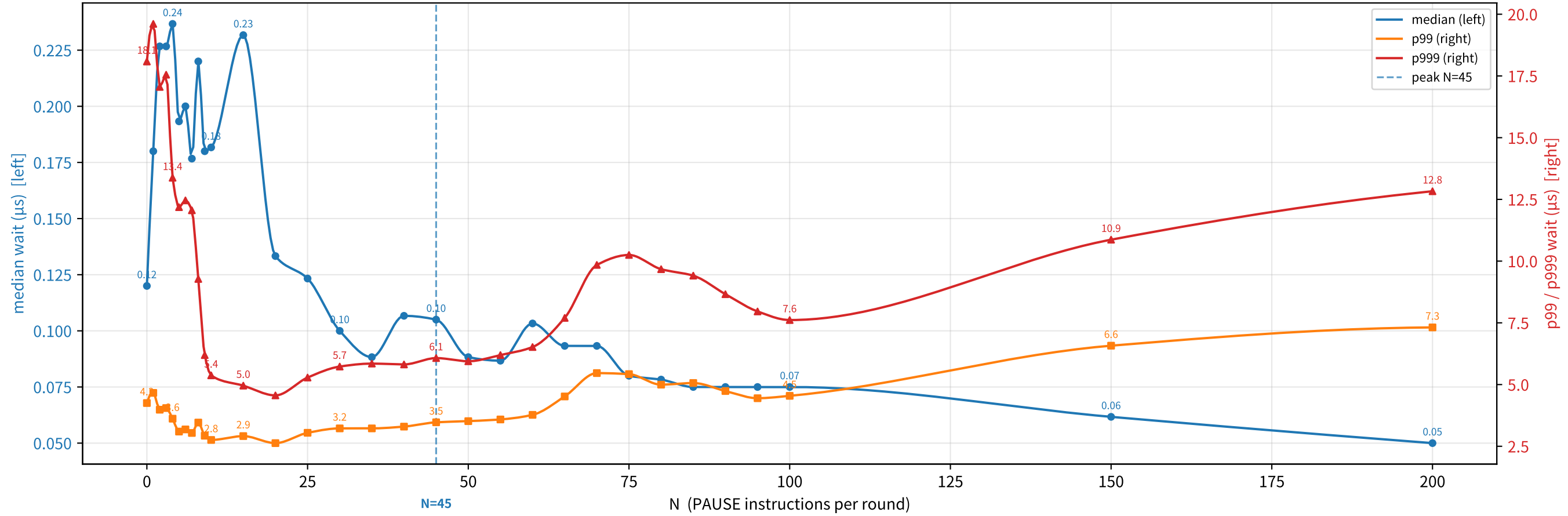
Ice Lake (sm110p, PAUSE~39cy) / TSC 2400 MHz
