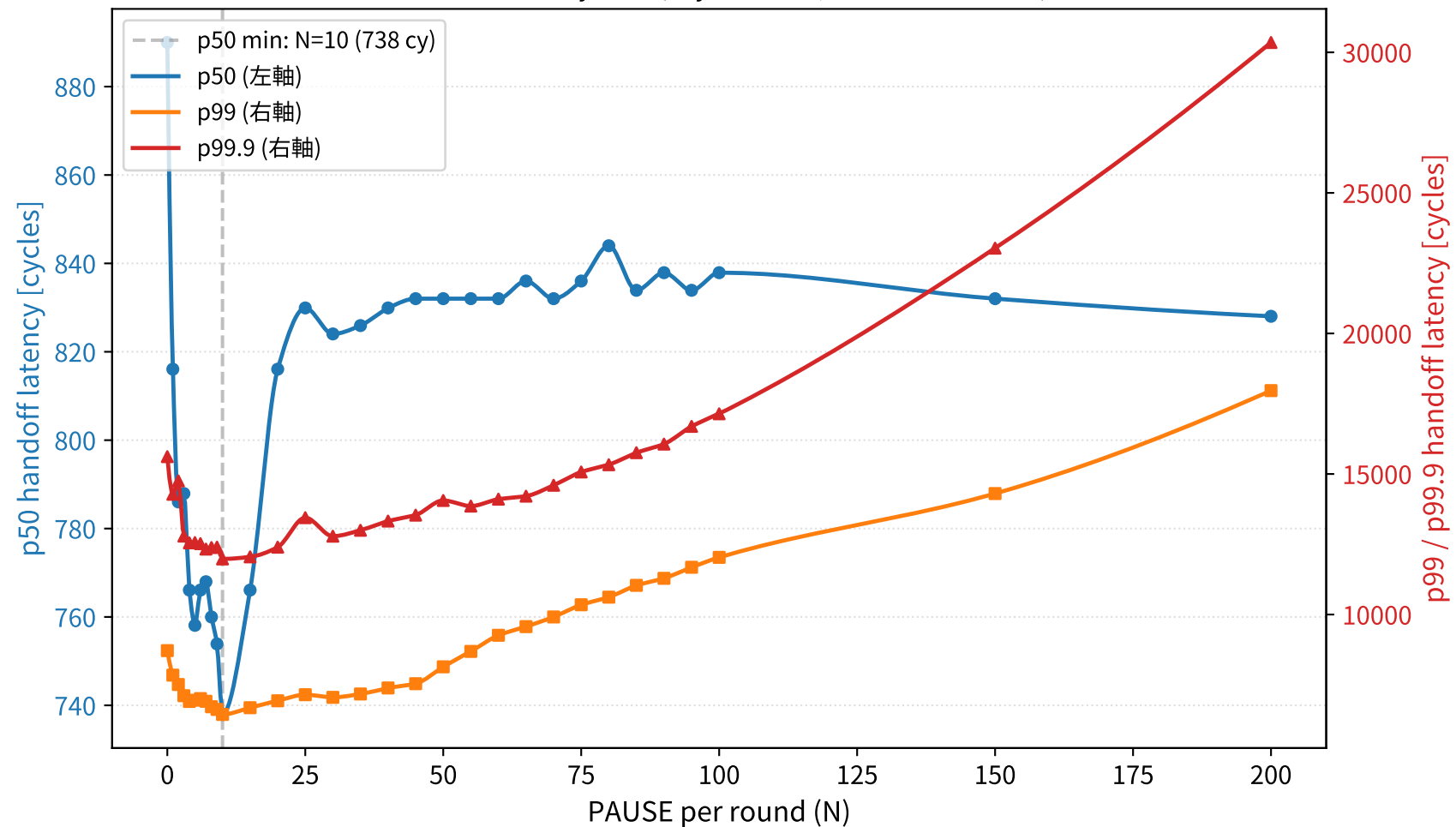
Handoff latency vs N (skylake ann, MC_THREADS=4)
