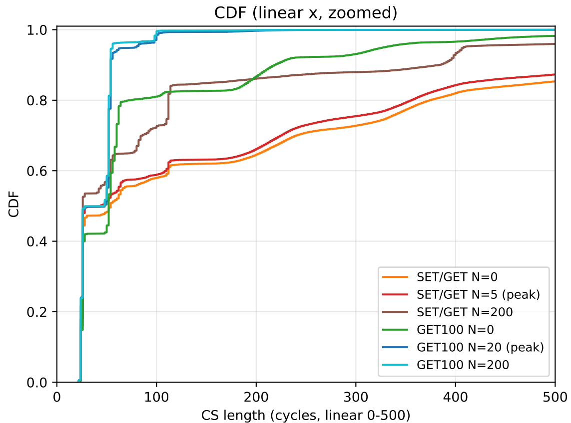
CS length CDF: SET/GET 50/50 vs GET 100% (skylake ann, T=4)
