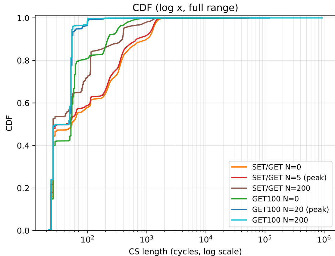
CS length CDF: SET/GET 50/50 vs GET 100% (skylake ann, T=4)
