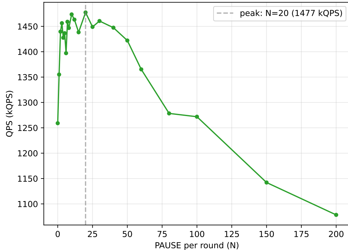
QPS vs N (GET 100%)
