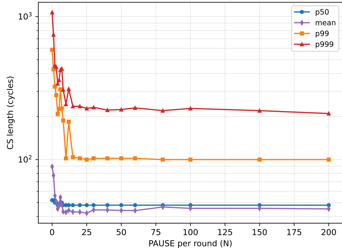
CS length percentiles (GET 100%)
