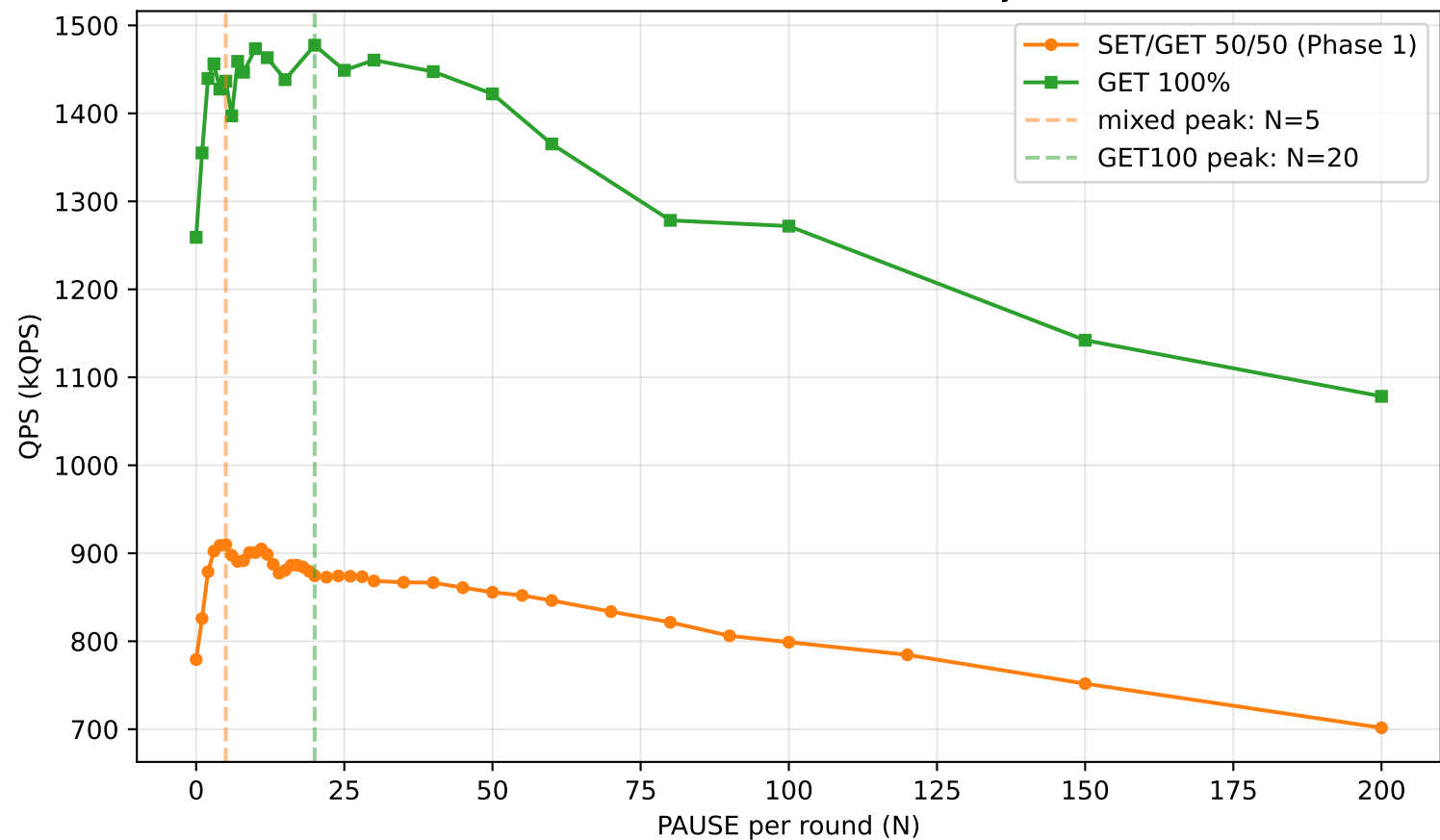
QPS vs N: SET/GET 50/50 vs GET 100% (skylake ann, T=4)
