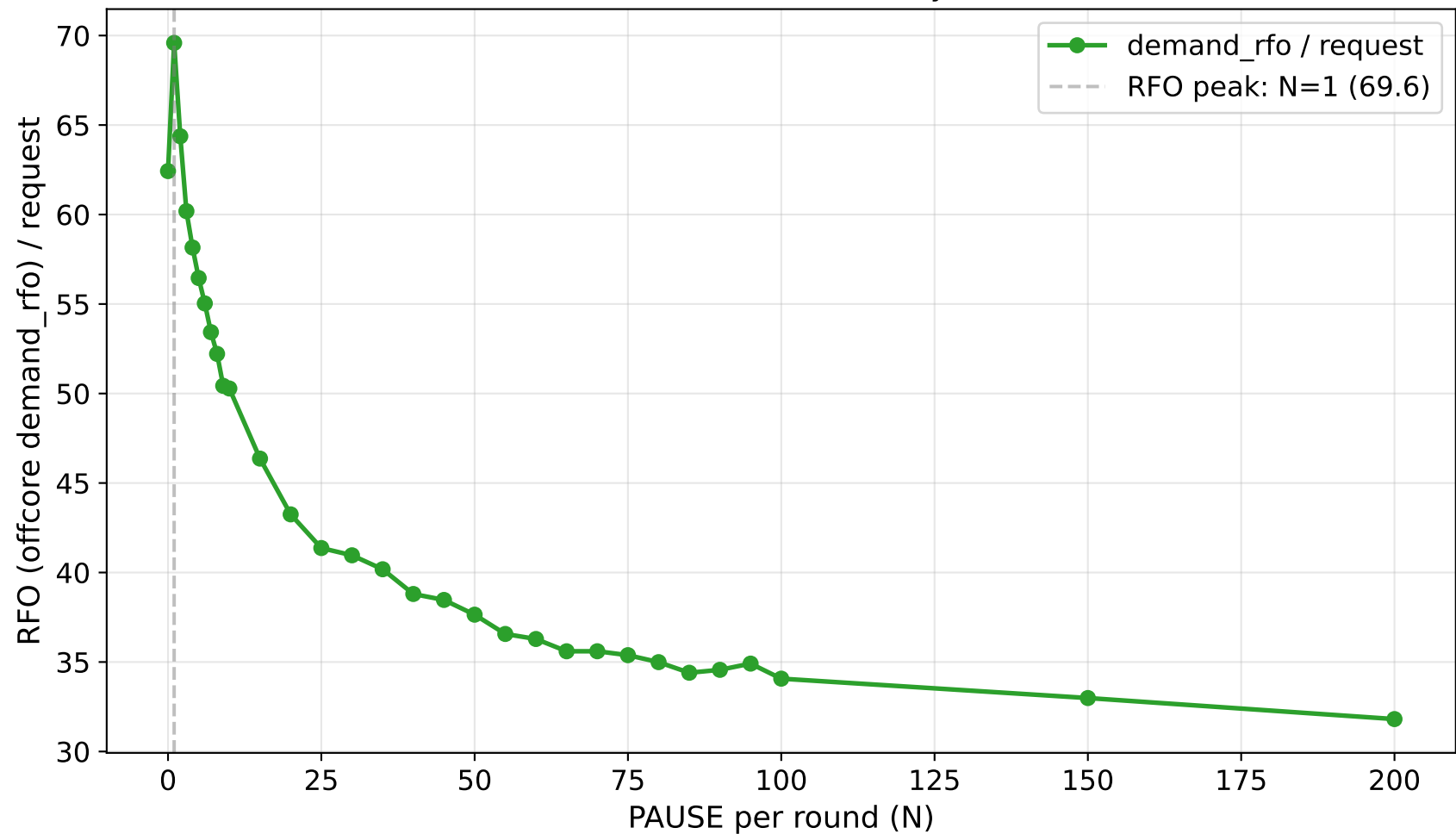
RFO (bus contention) vs N (skylake ann)
