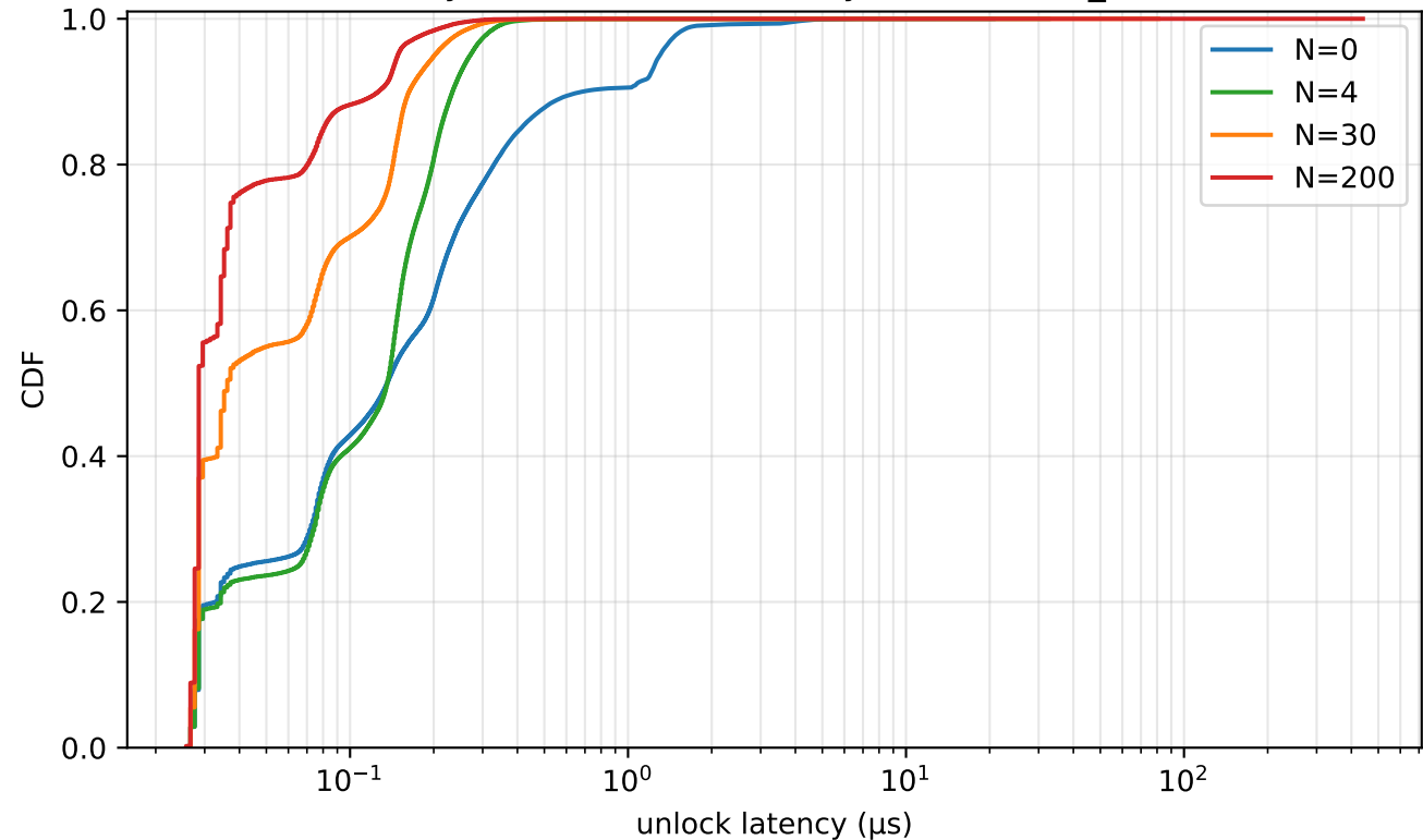
unlock latency CDF (selected N) (skylake ann, MC_THREADS=4)
