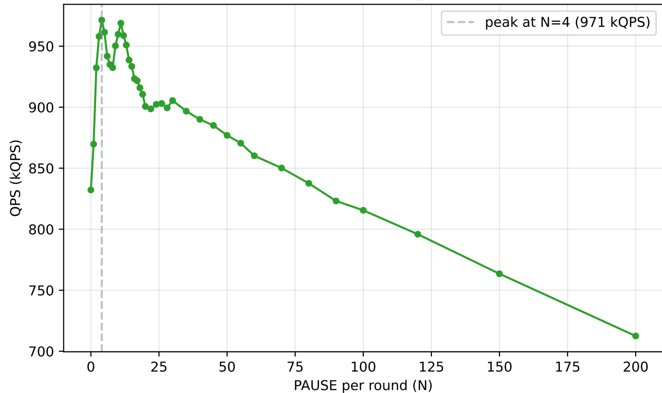
QPS vs N (skylake ann, MC_THREADS=4)
