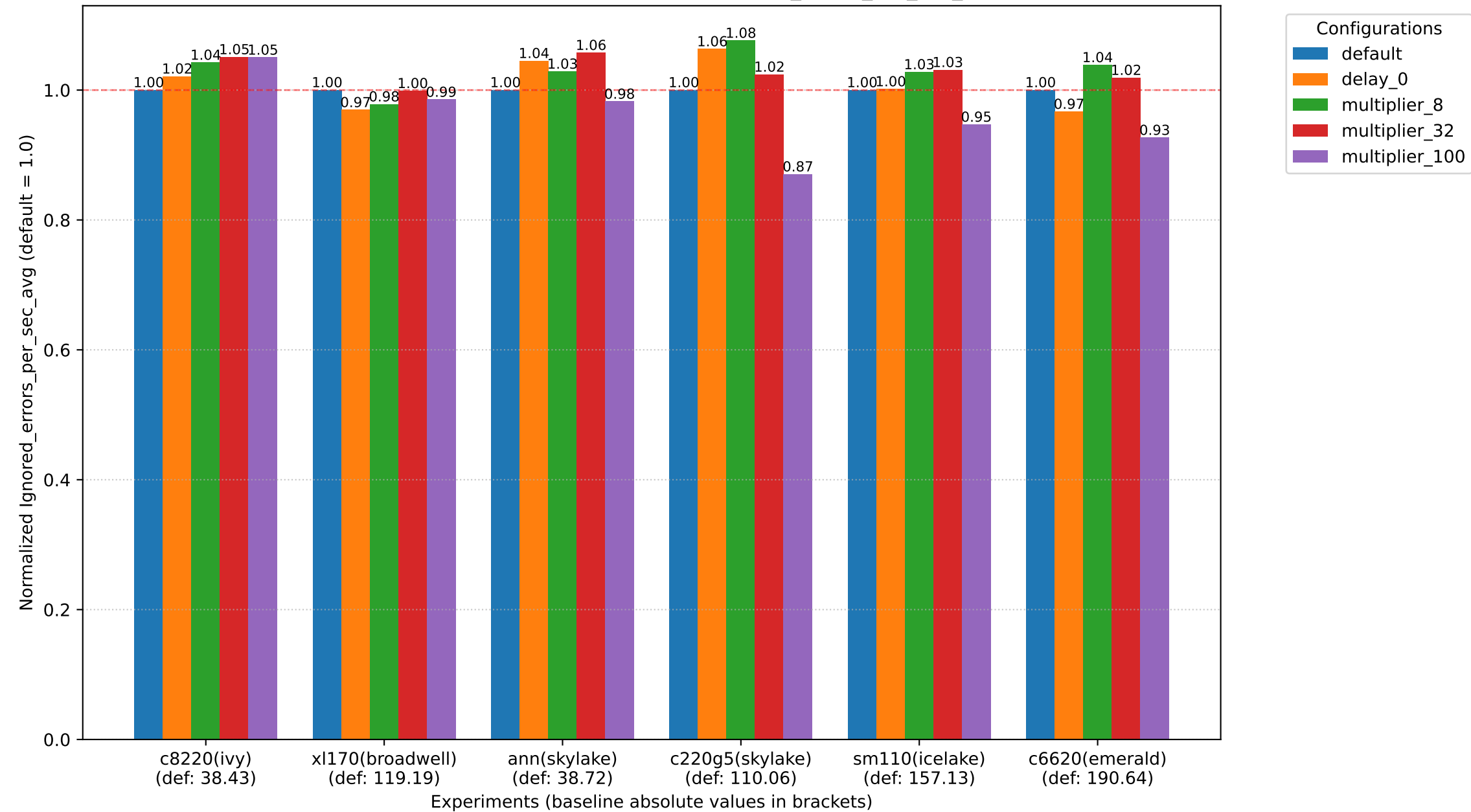
not consolidated sysbench 16threads - Ignored_errors_per_sec_avg
