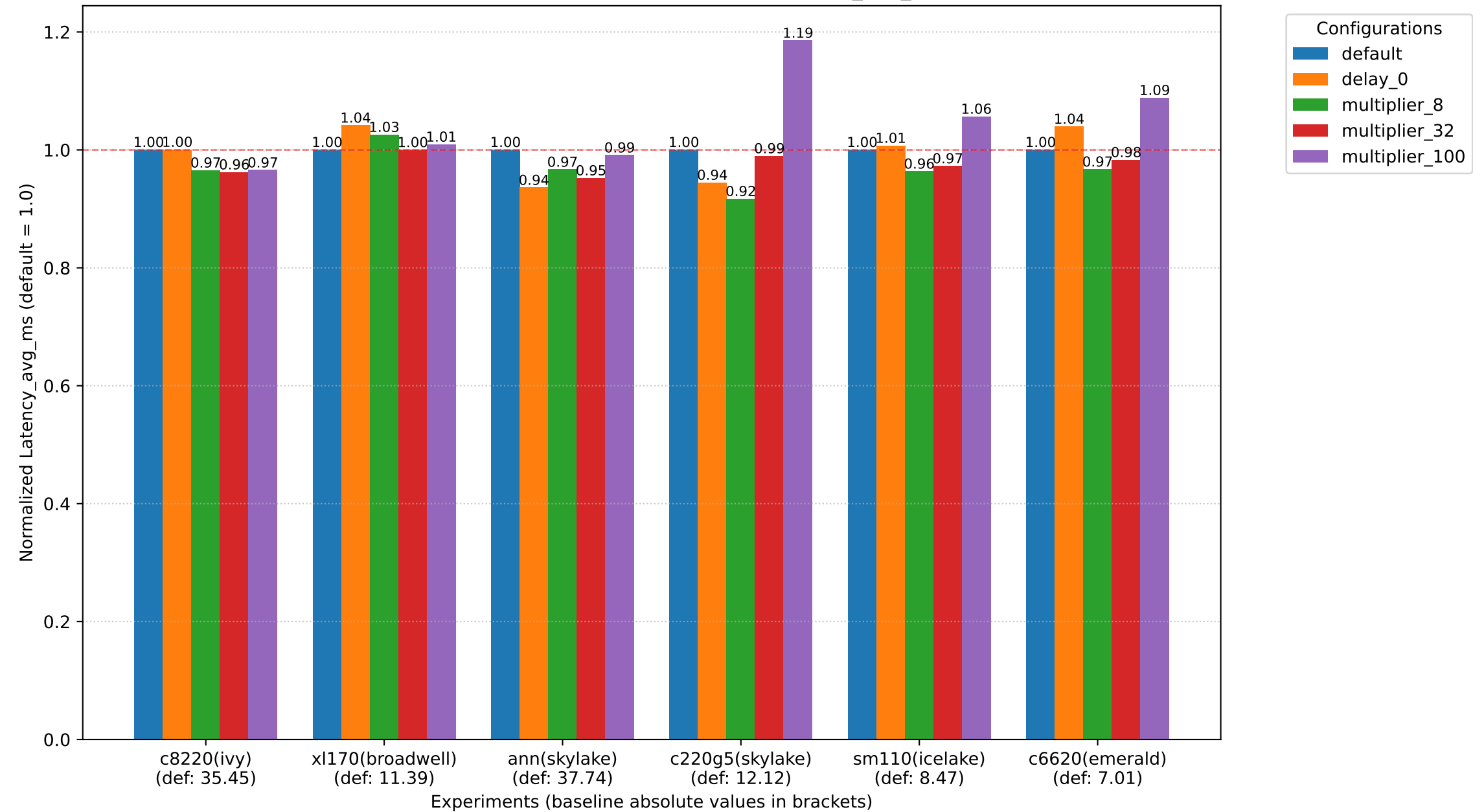
not consolidated sysbench 16threads - Latency_avg_ms
