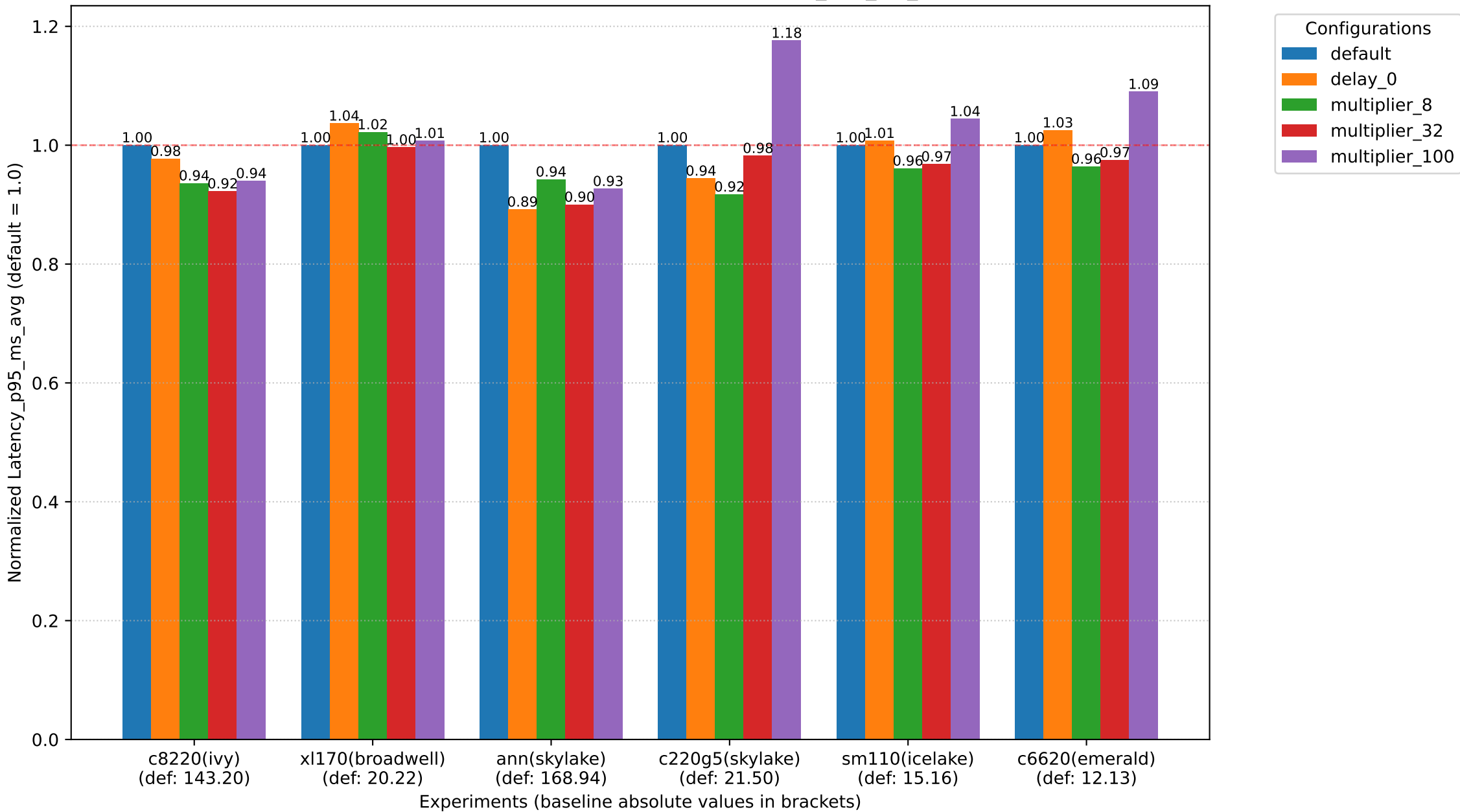
not consolidated sysbench 16threads - Latency_p95_ms_avg
