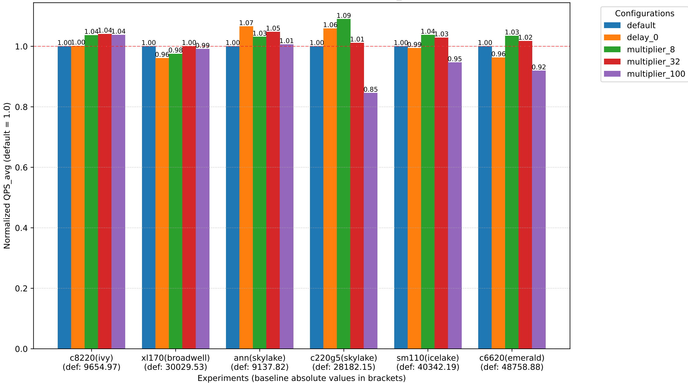
not consolidated sysbench 16threads - QPS_avg
